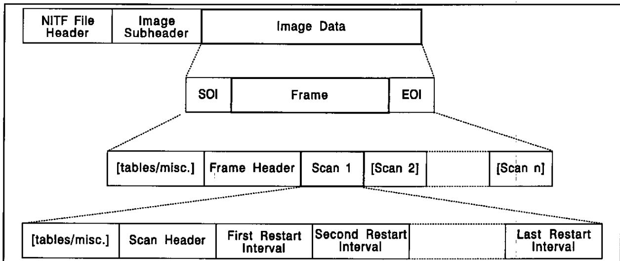
FIGURE 7. NITF single block file structure (IMODE=B or P).
