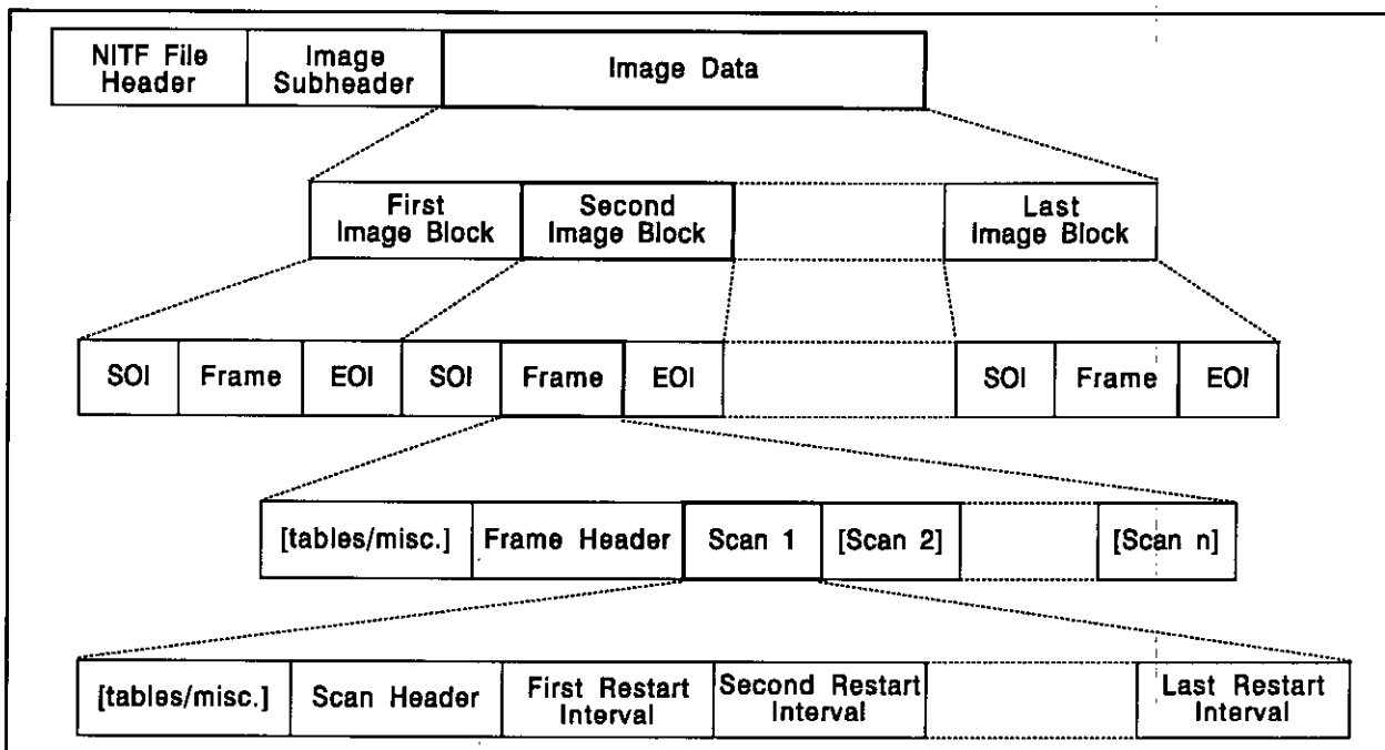
FIGURE 8. NITF multiple block file structure (IMODE=B or P).
