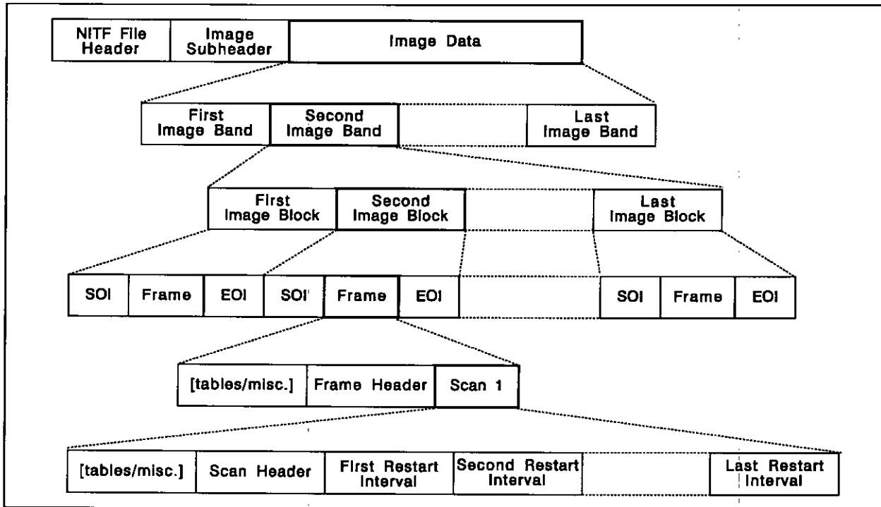
FIGURE 9. NITF multiple block file structure (IMODE=S).
