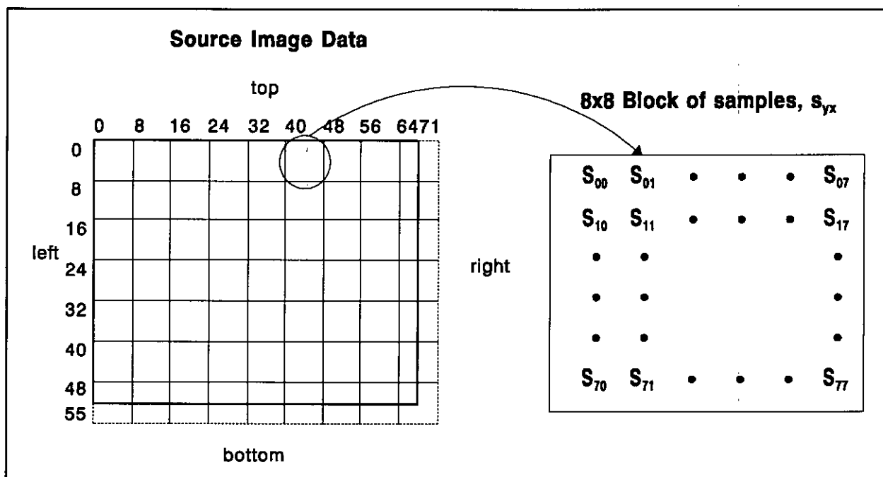
FIGURE 2. Partitioning an example source image with 52 lines and 68 samples into 8x8 blocks.
