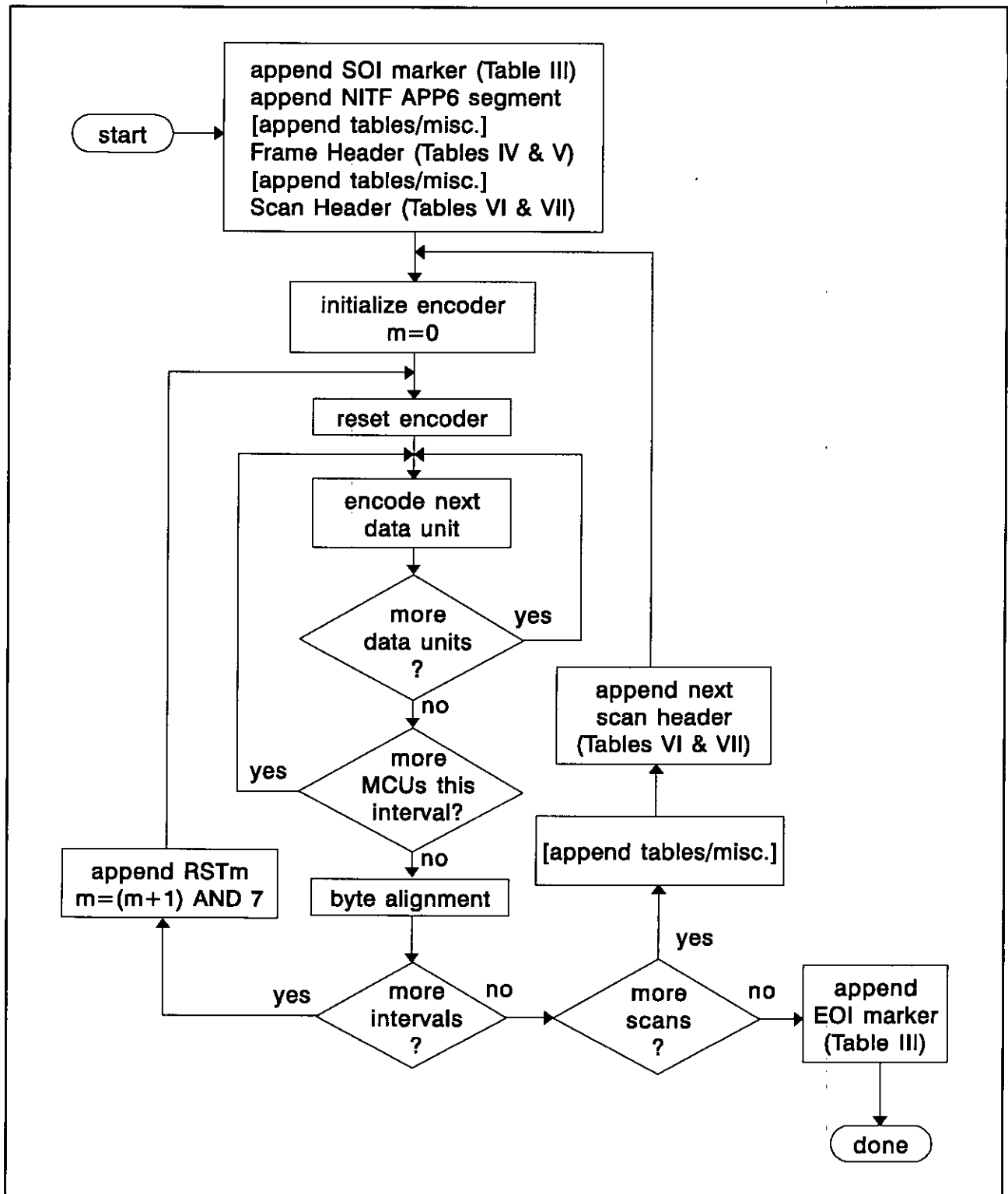
FIGURE 5. Simplified encode flow chart.
