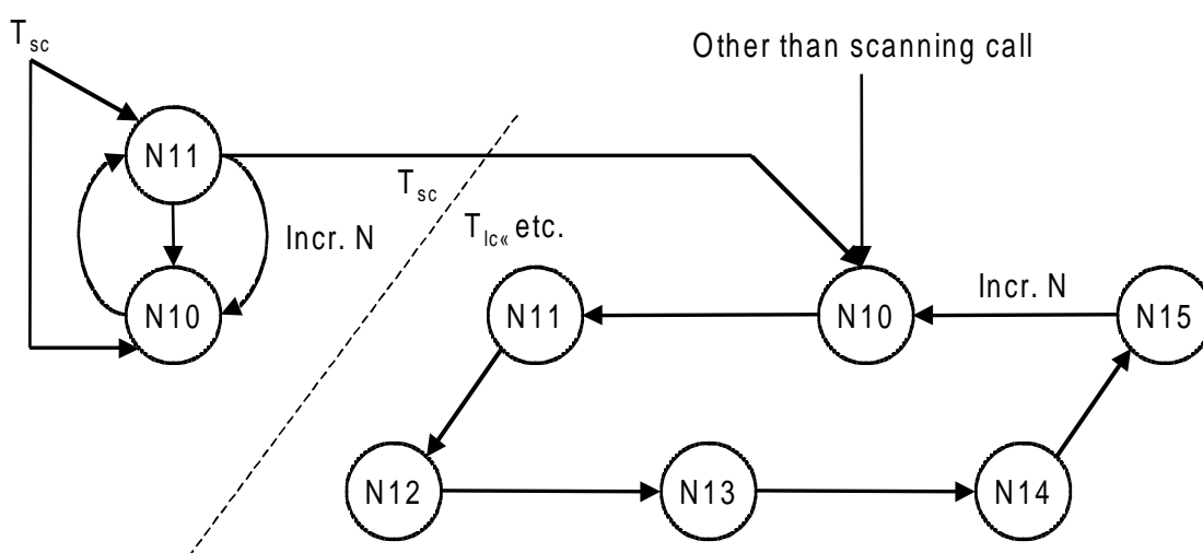
b. Transmitting station state diagram (2 second PI)
