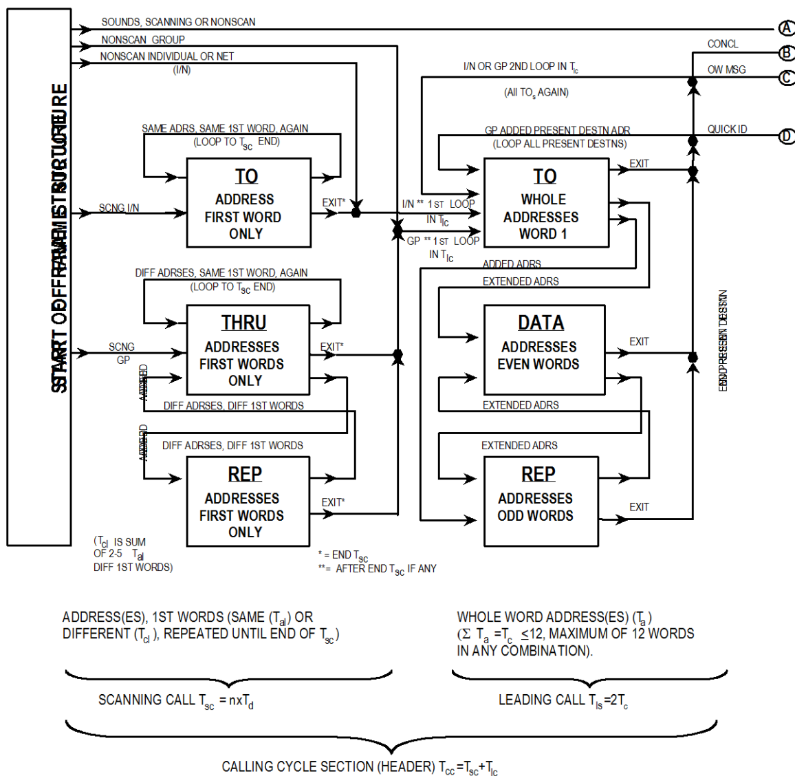
FIGURE A-18. Valid word sequence (calling cycle section).
