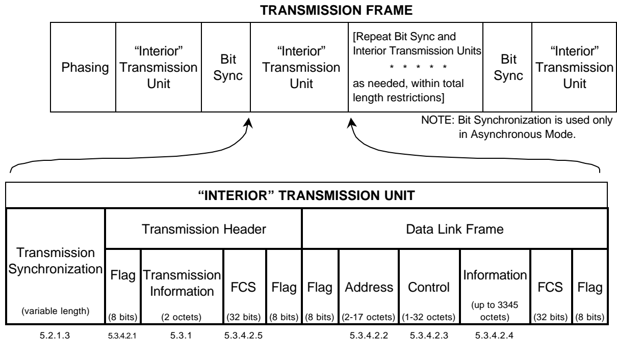
FIGURE 23. Physical-layer concatenation.
