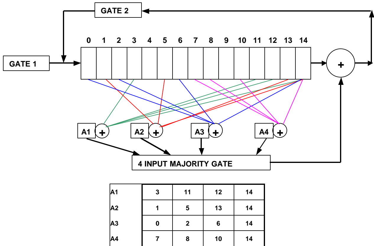
FIGURE 99. BCH (15, 7) majority logic decoding.
