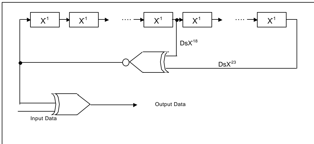
FIGURE 89. Data scrambler structure.
