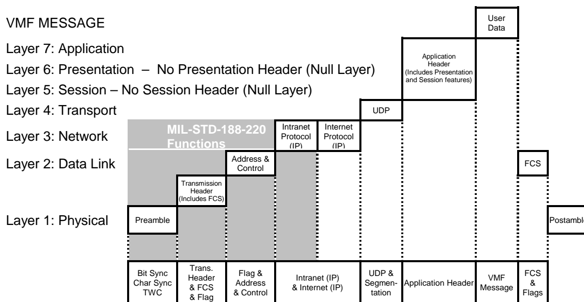
FIGURE 50. PDU construction.
