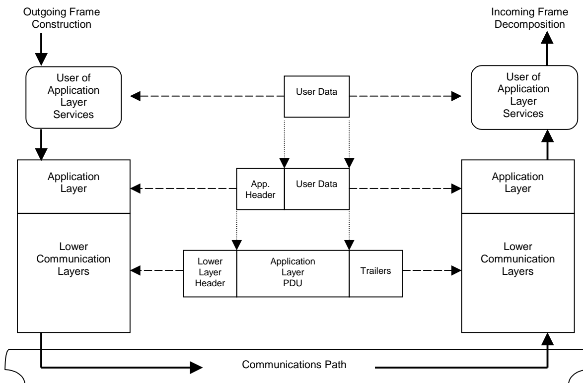
FIGURE 54. Application layer interaction with other communication layers.
