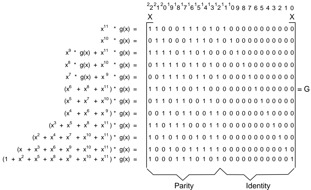
FIGURE 48. Generator matrix G.
