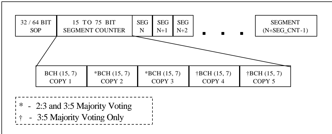
FIGURE 90. Multi-dwell packet.
