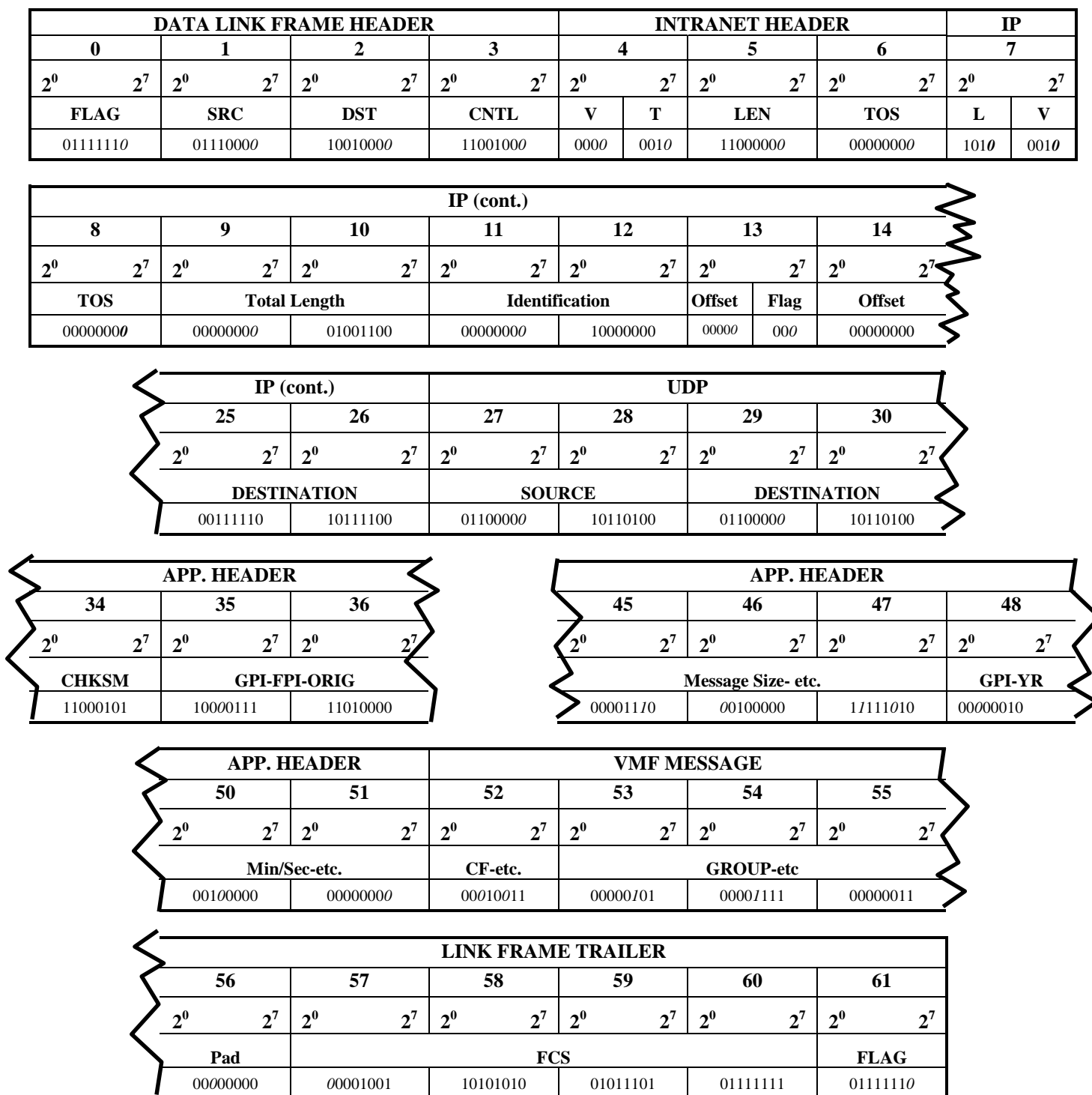
FIGURE 71. Serial representation of data link layer PDU.
