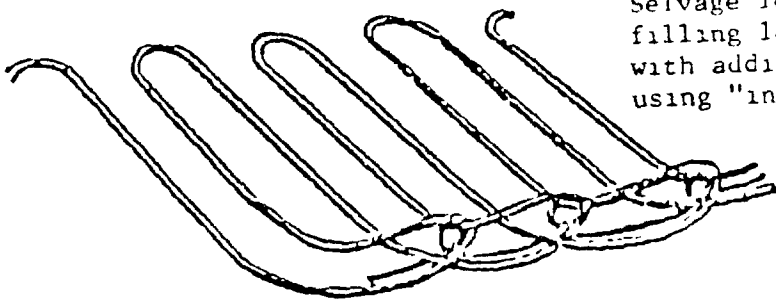
FIGURE 1 - CATCH-CORD DIAGRAM (SHUTTLELESS CONSTRUCTION)
