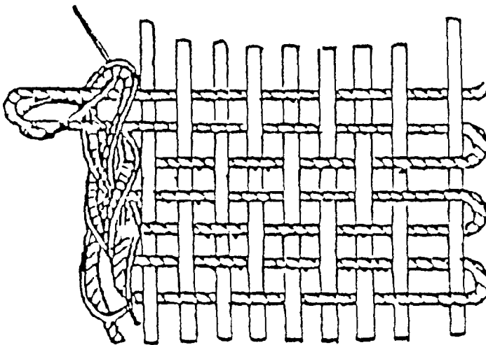
FIGURE 2 - CATCH-CORD DIAGRAM (SHUTTLELESS CONSTRUCTION)
