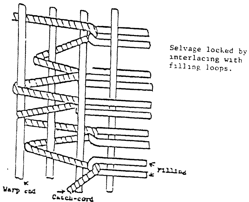
FIGURE 3 - CATCH-CORD DIAGRAM (SHUTTLELESS CONSTRUCTION)
