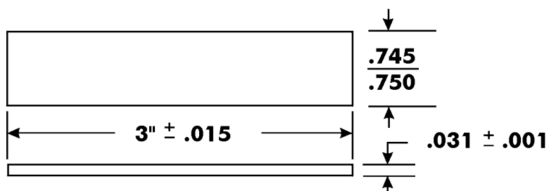
FIGURE 3. Test Strip N. 1/
