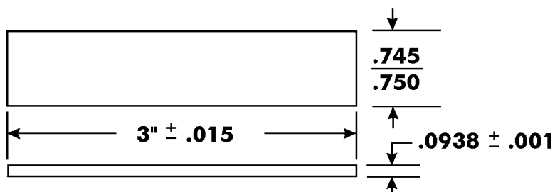
FIGURE 2. Test Strip C. 1/
