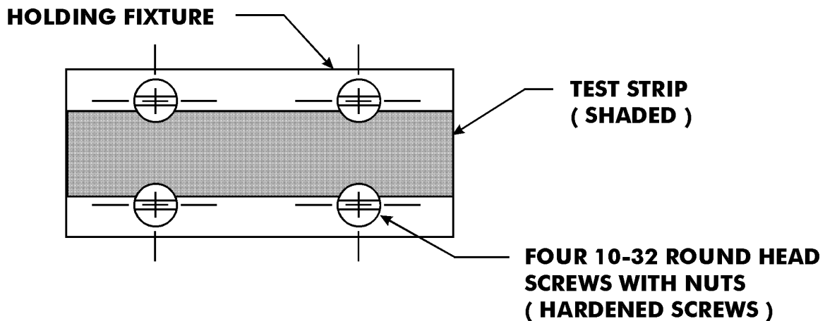
FIGURE 5. Assembled test strip and holding fixture.
