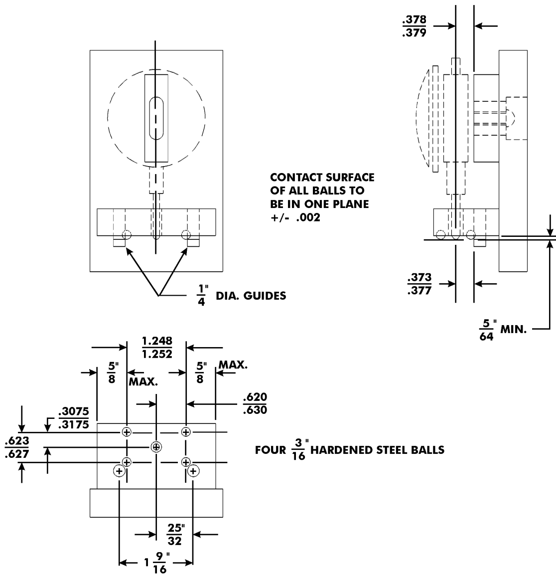
FIGURE 6. Test gauge.
