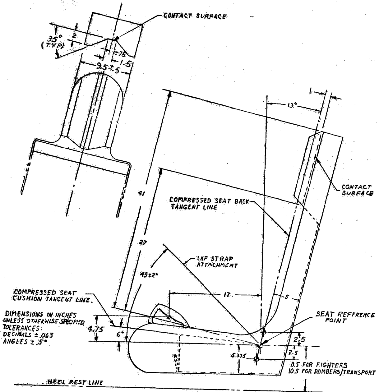
FIGURE 1. Side View of Seat with Example of Headrest Details
