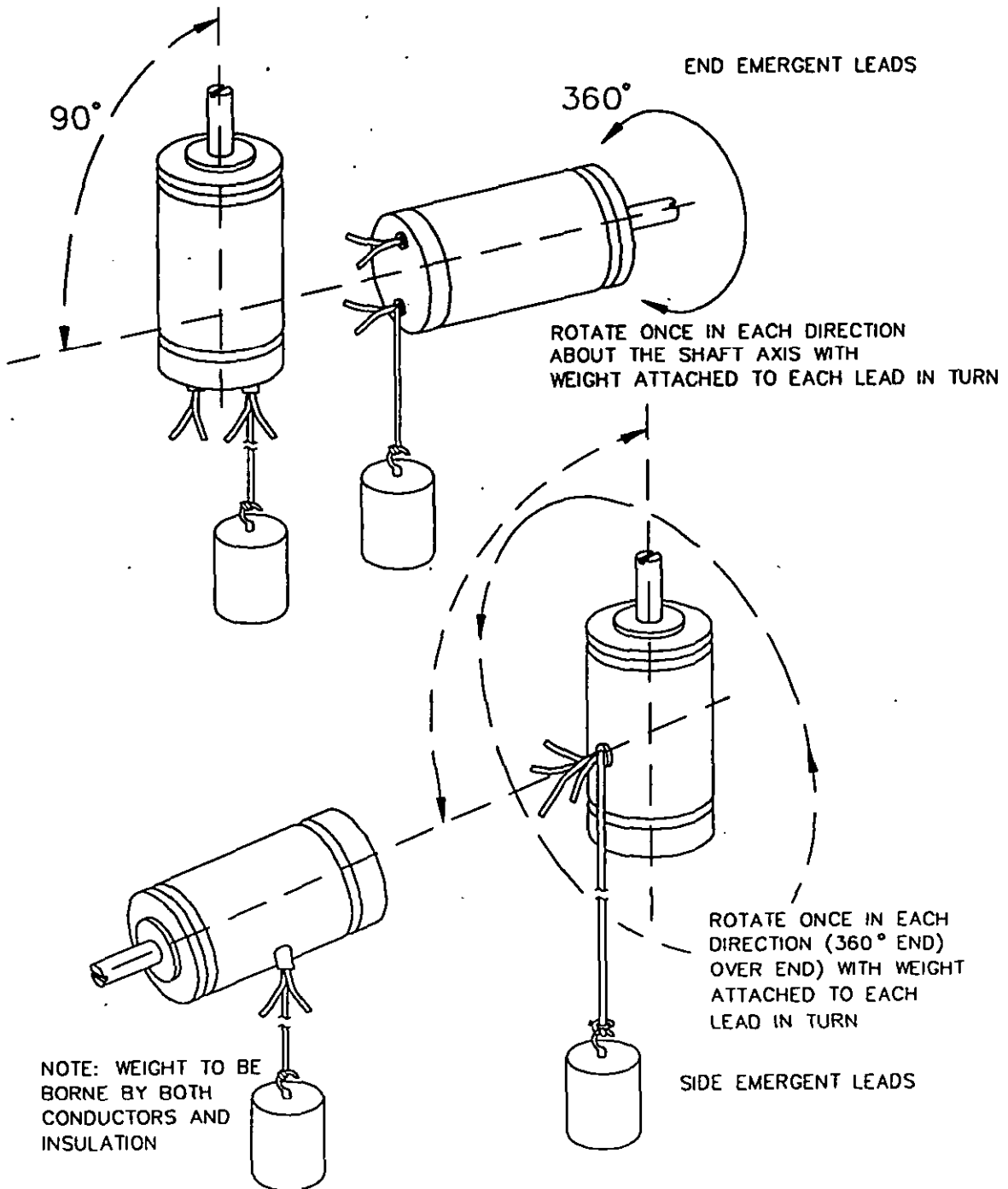
FIGURE 14. Lead wire stress test.
