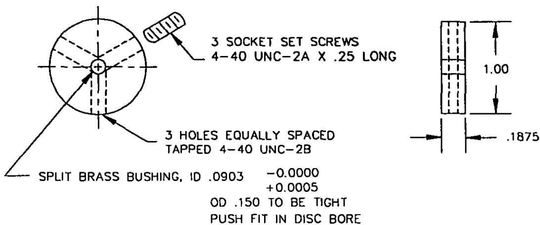
FIGURE 1B. Standard disc for loading size 05 and 08 servocomponent shaft.
