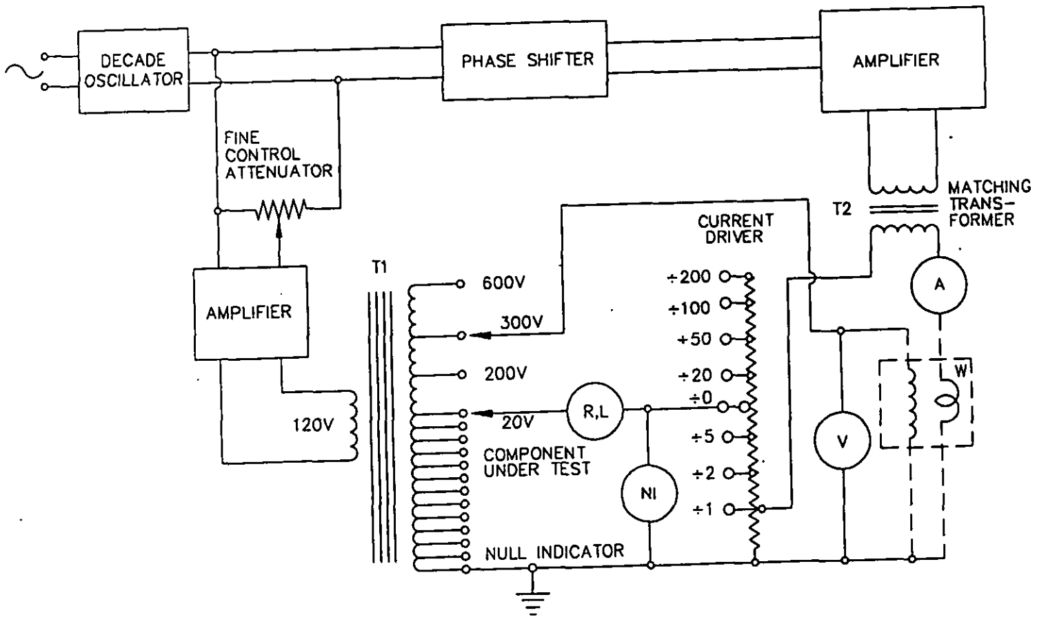
FIGURE 9. Marshall potentiometer.
