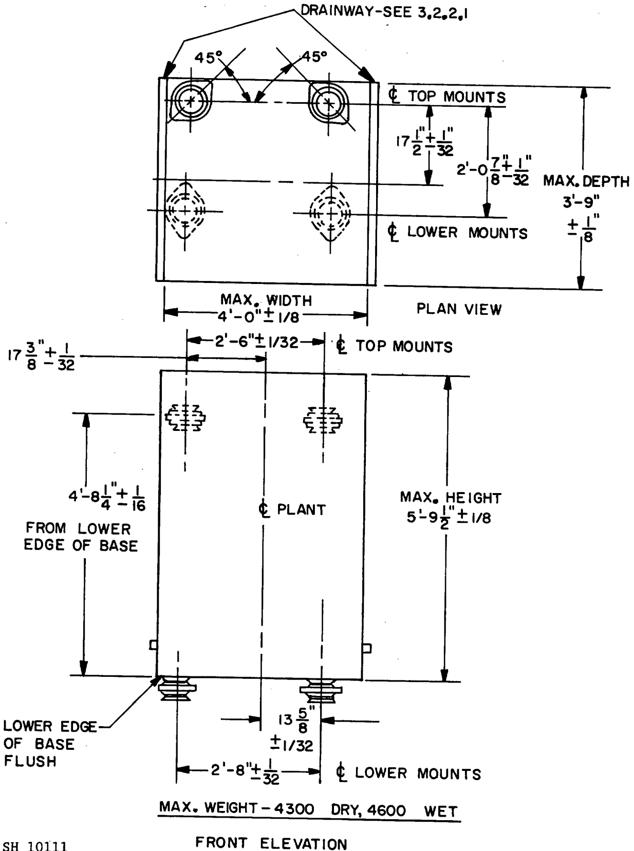
FIGURE 1. Weight, overall dimensions and mount location.
