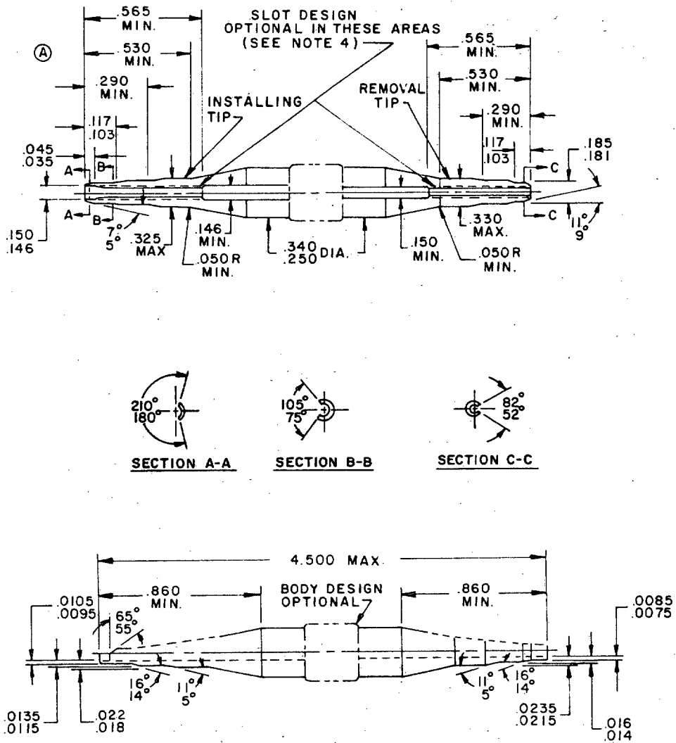
FIGURE 2. Installing and removal tool, dash -03.
