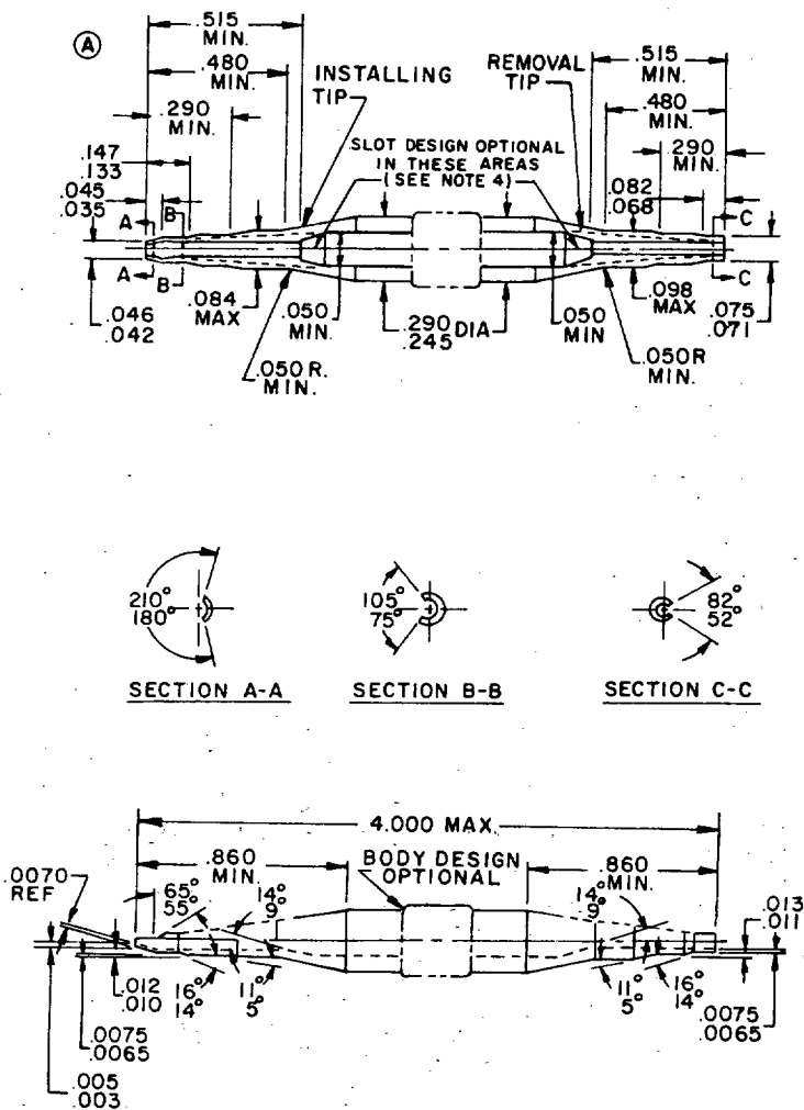
FIGURE 3. Installing and removal tool, dash -04.
