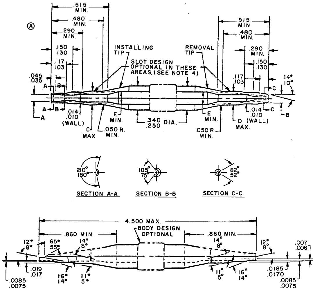
FIGURE 1. Installing and removal tool, dash -01 and -02.
