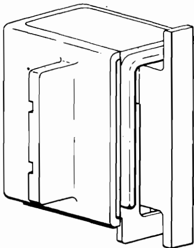
FIGURE 2. Installation procedures for left-hand or right-hand hinged armored doors swinging out to open, style 2.
