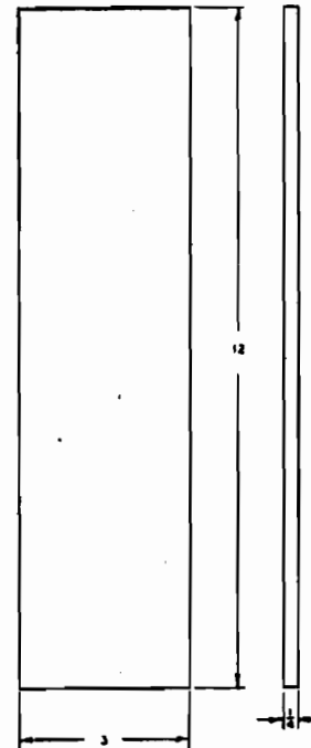
13 DETAIL 26B MOUNTING PLATE MATL: 304 STAINLESS STEEL NO. RECD: 1 PER APPL. STYLE
