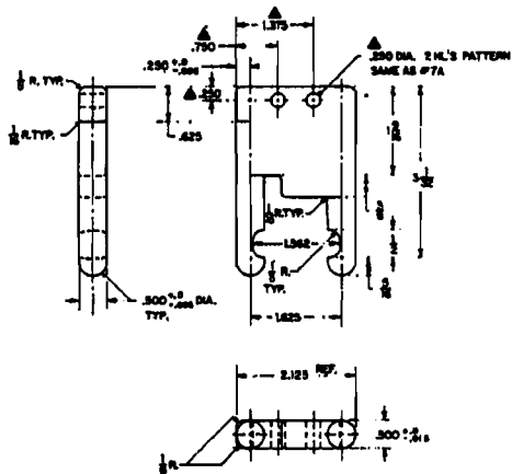
7B DETAIL 22A SHACKLE PIN FOR SCISSOR WITH 1/2 # SHACKLE REMOVED MATL. 304L NO. REQD: 2 PER STYLE
