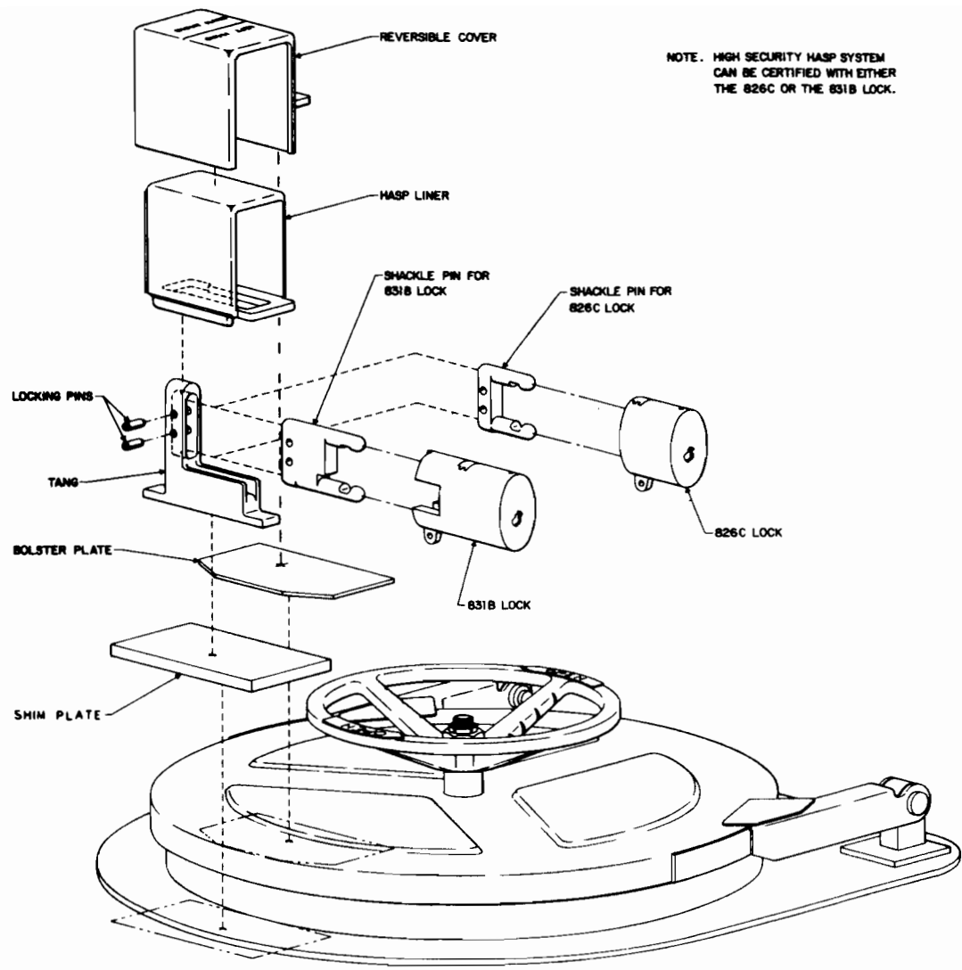
18-21 OR 25" DIA. QUICK ACTING WATER TIGHT SCUTTLE
