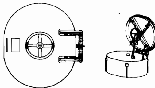
QUICK ACTING WATER TIGHT RAISED HATCH (24 X 30 SHOWN)
