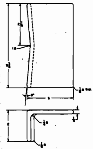
4 DETAIL 9E TAMPER BRACKET MATL. 304 L NO. REQD: 1 PER APPL. STYLE
