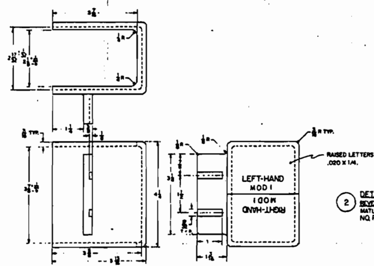
FIGURE 1. High security hasp, shipboard configuration and parts list. - Continued
