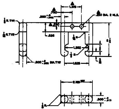
7A DETAIL 22E SHACKLE PIN FOR SCISSOR LOCK / 1/2 # SHACKLE REMOVED MATL. 304L NO. REQD: 1 PER STYLE
