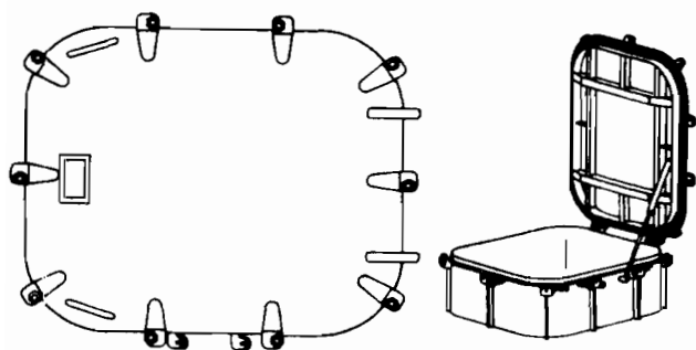
INDIVIDUALLY DOGGED RAISED HATCH (30 X 36 SHOWN)
