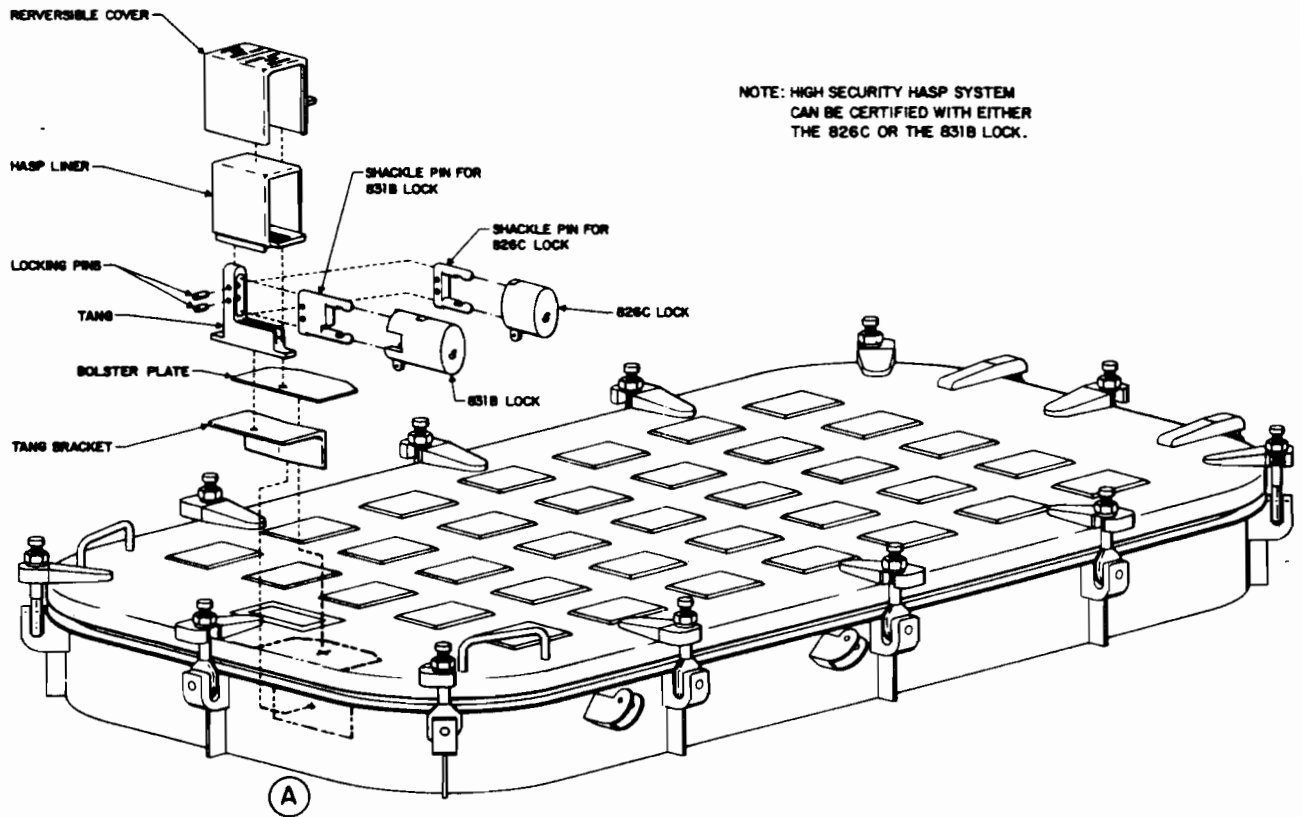
INDIVIDUALLY DOGGED RAISED HATCH 30 X 60 SHOWN
