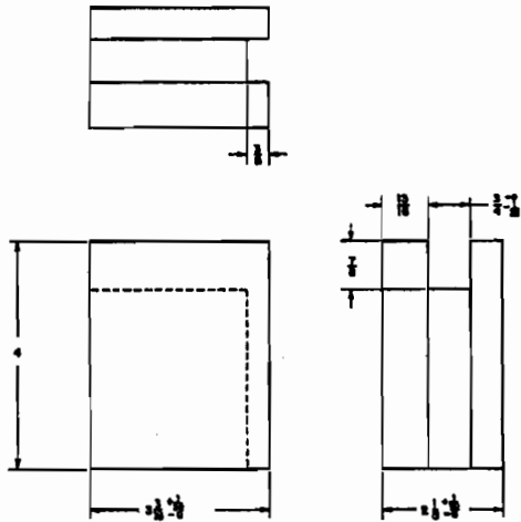
11 DETAIL 30D FOAM INSTALLATION JIG MATL: POLYETHYLENE L7 TO 2.0/FT. 3 DENSITY (HOT WIRE CUT PERMISSIBLE) NO. RECD 1 PER STYLE
