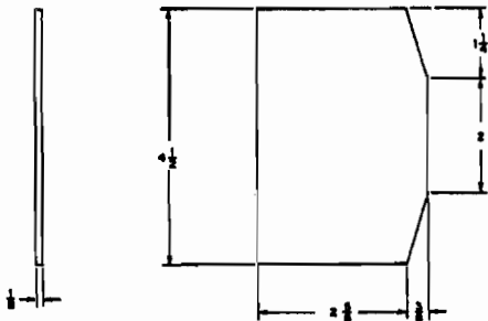
10 DETAIL 31A BOLSTER PLATE MATL: ASTM A36 PLATE NO. RECD 1 PER APPL. STYLE
