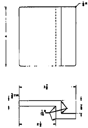
9 DETAIL 17B 1/2" BRACKET FOR INWARD OPENING CABINET DOORS MATL. 304L NO. REQD: 1 PER APPL. STYLE
