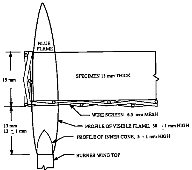
FIGURE 3. Relative positions of burner wing top, flame, specimen, and specimen support.
