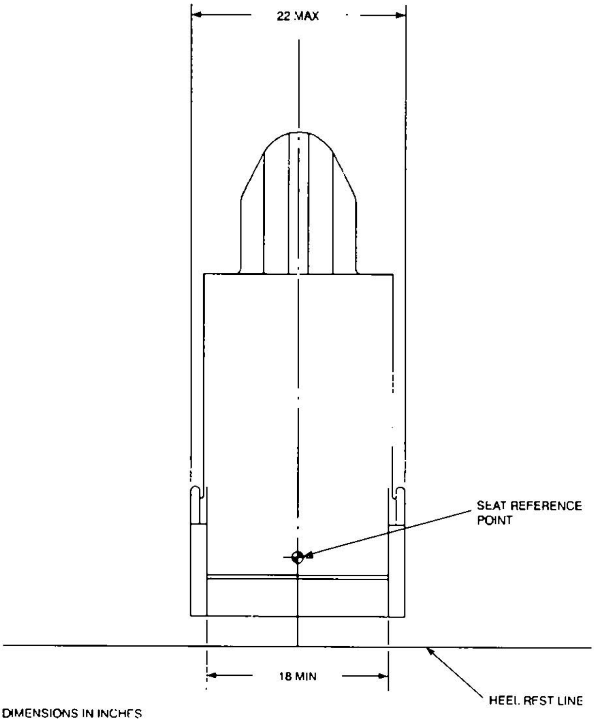
FIGURE 3. Front view of seat.
