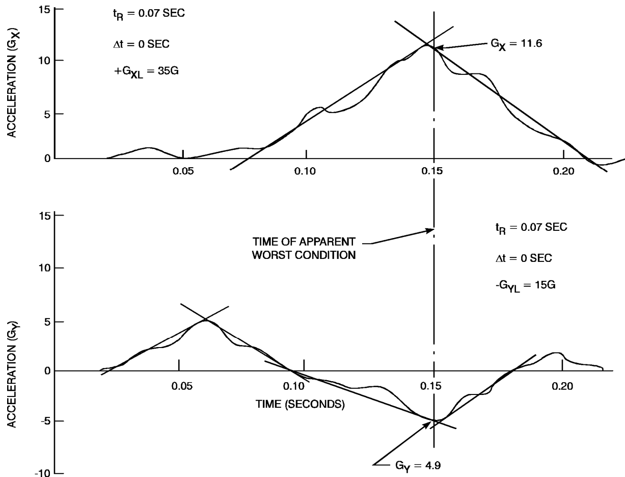
FIGURE 11. Multiaxial acceleration environment example.
