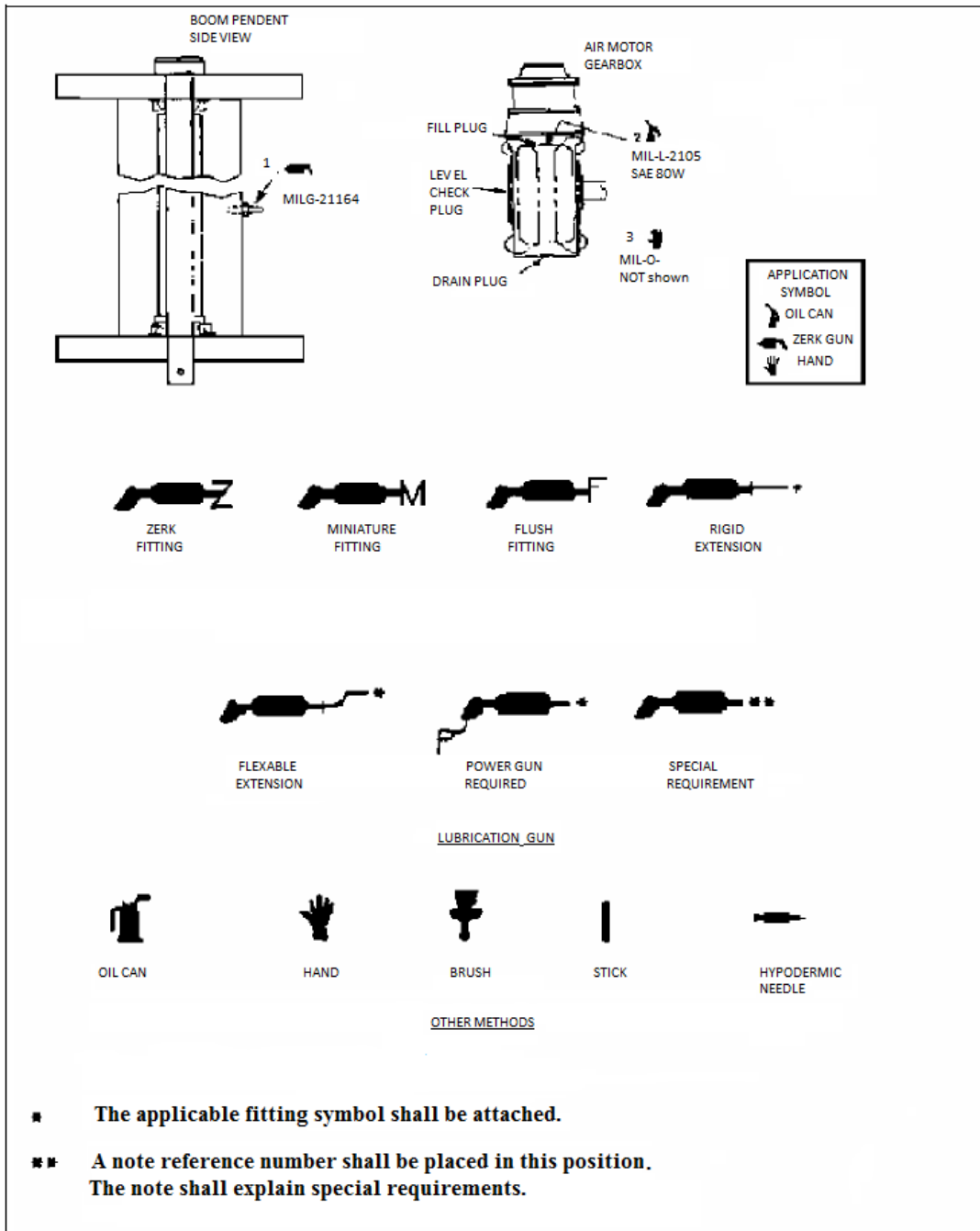
FIGURE 2. Sample of lubrication and illustration symbols
