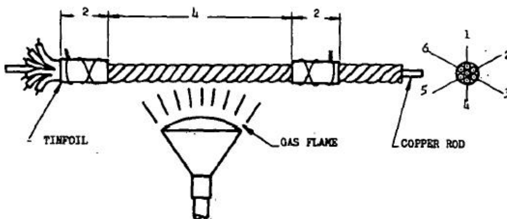
FIGURE 1. Flammability test, procedure I.
