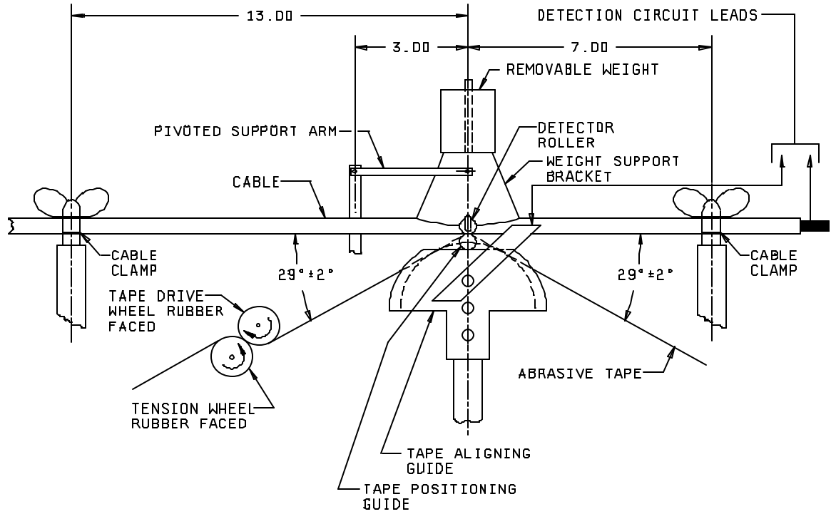
FIGURE 1. Assembly sketch of abrasion tester.
