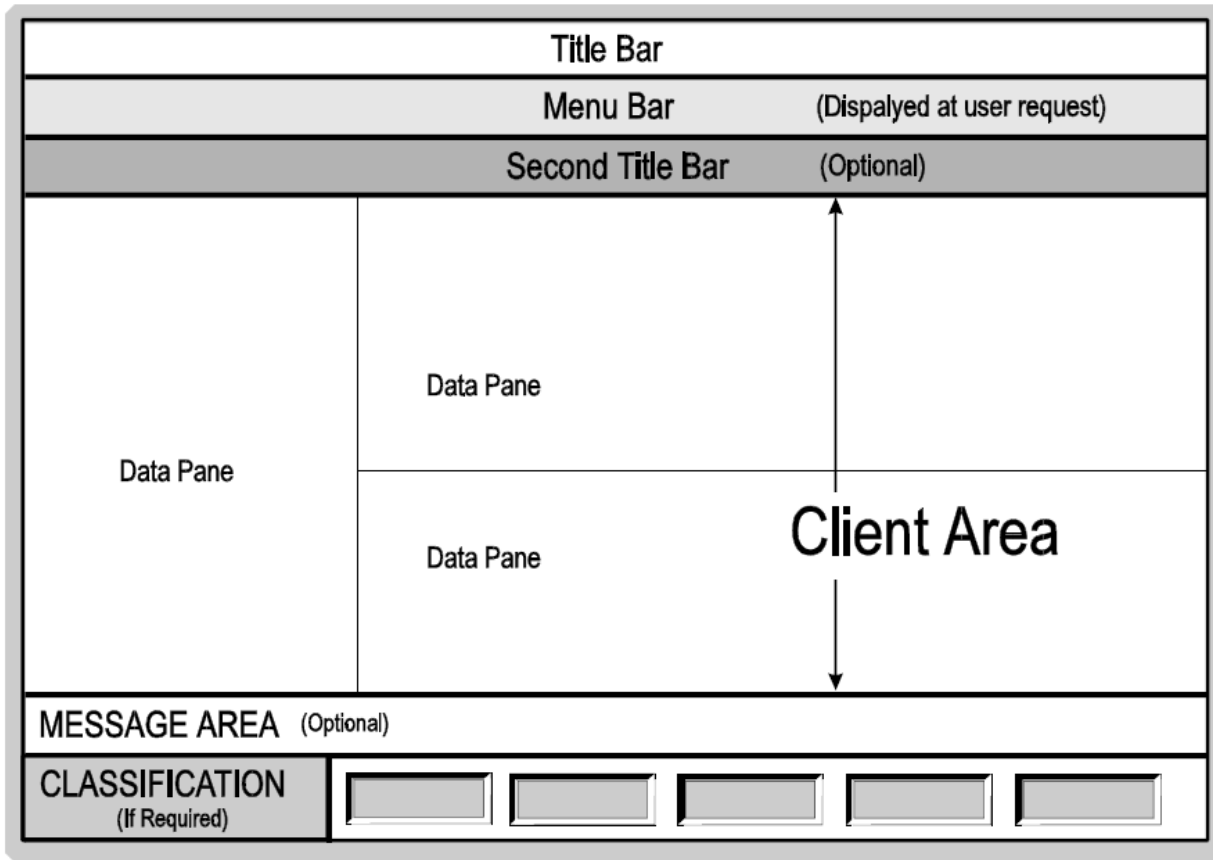
FIGURE 4. Client area components..
