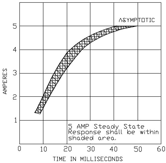
FIGURE 4. Response (current versus time) type I inductors only.
