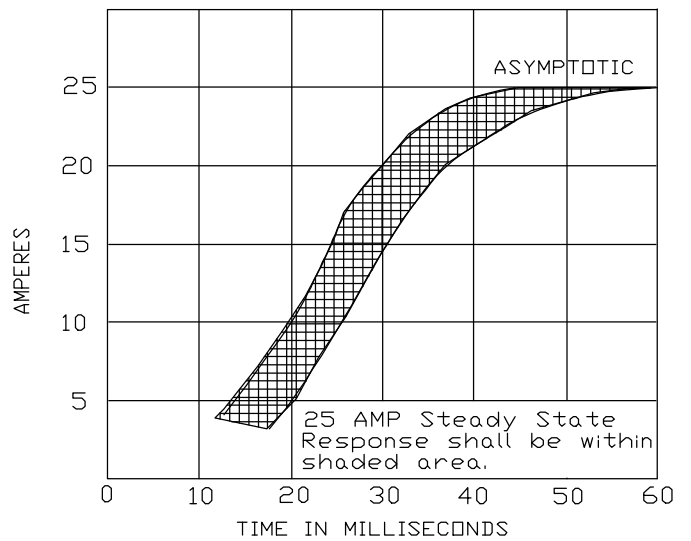
FIGURE 4. Response (current versus time) type I inductors only.
