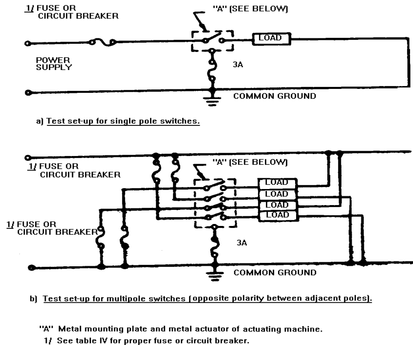
FIGURE 2. Test set-up for electrical endurance test.
