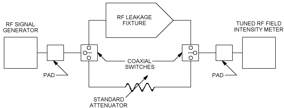
SCHEMATIC TEST SYSTEM
