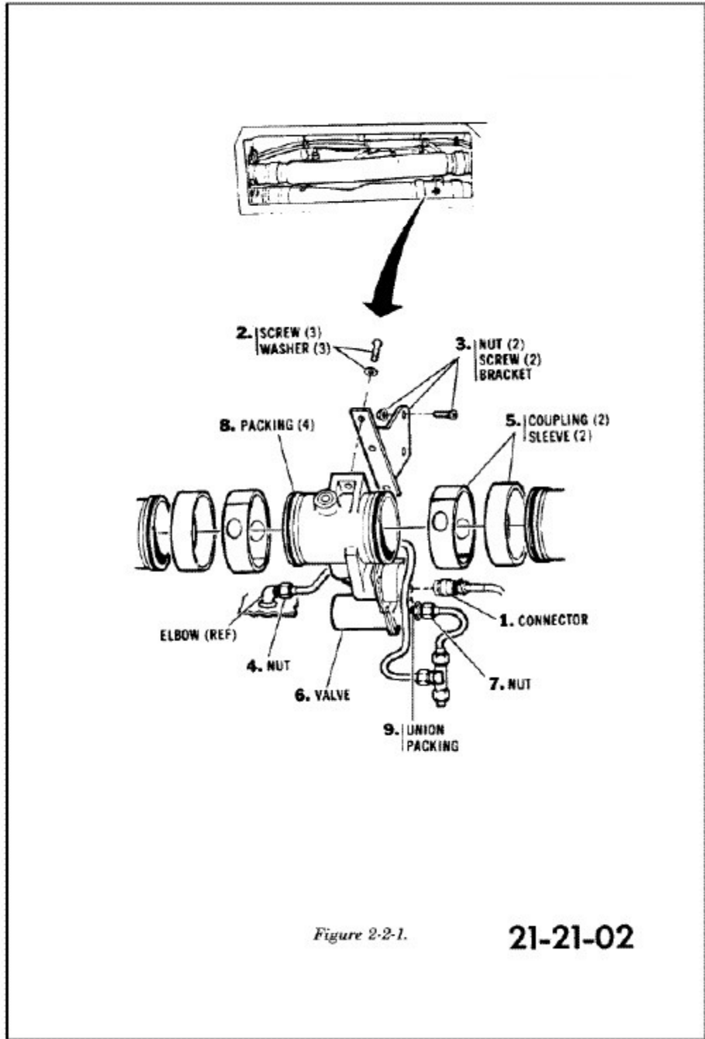
FIGURE 3. Example job guide task - Continued.
