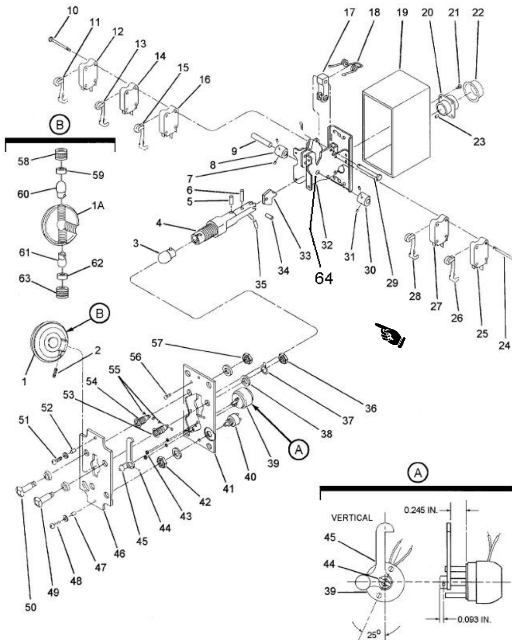
Figure 1. Landing Gear Control Panel - Disassembly/Assembly
