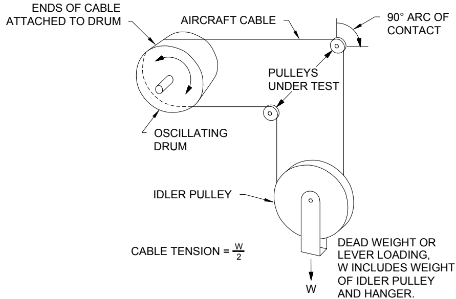
FIGURE 2. Endurance test setup.
