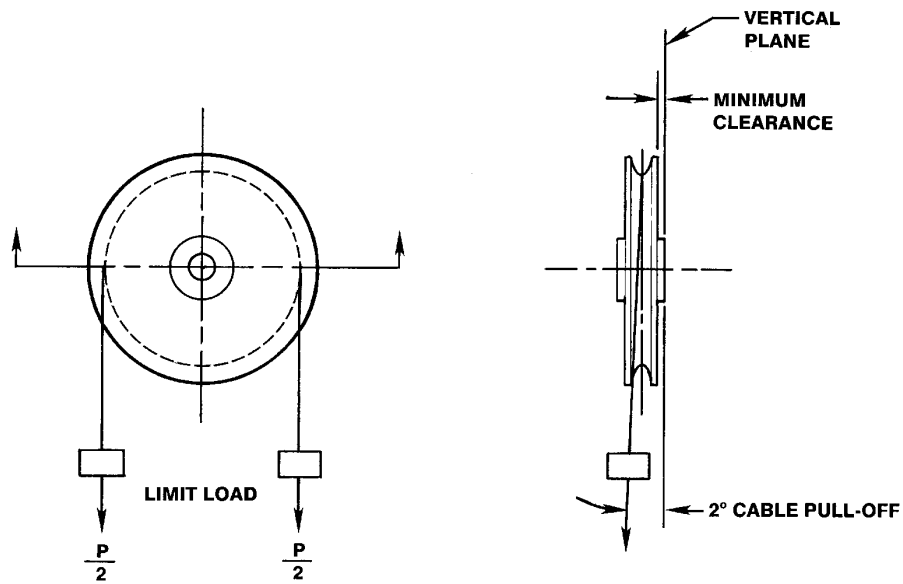
FIGURE 3. Wobble clearance test setup.
