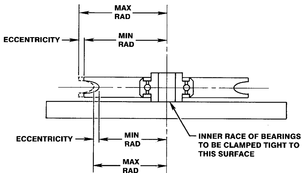
FIGURE 1. Eccentricity test setup.
