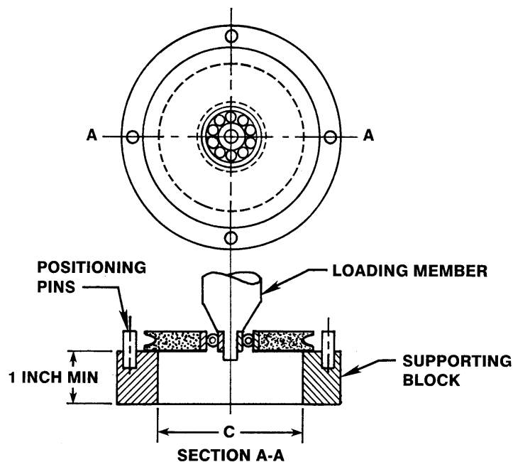
FIGURE 4. Bonding strength test setup.
