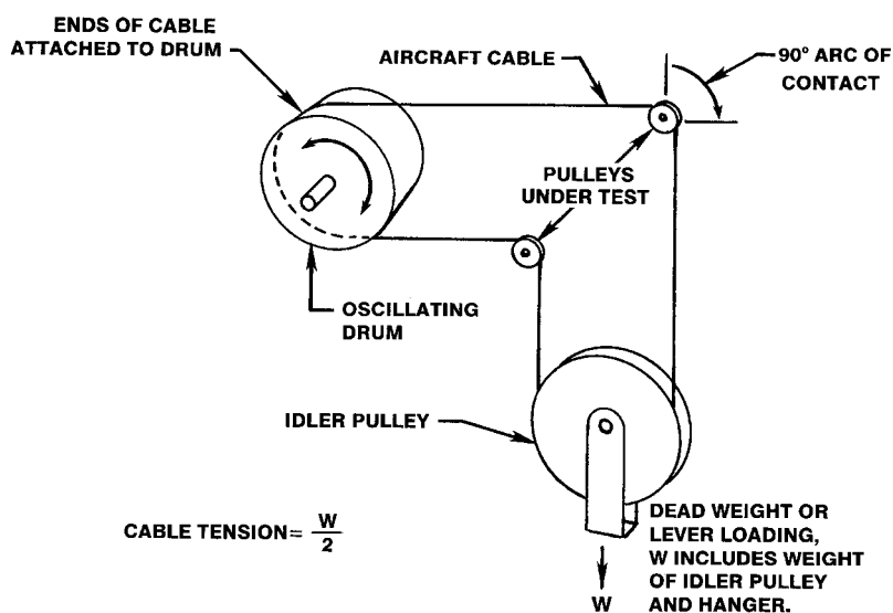
FIGURE 2. Endurance test setup.
