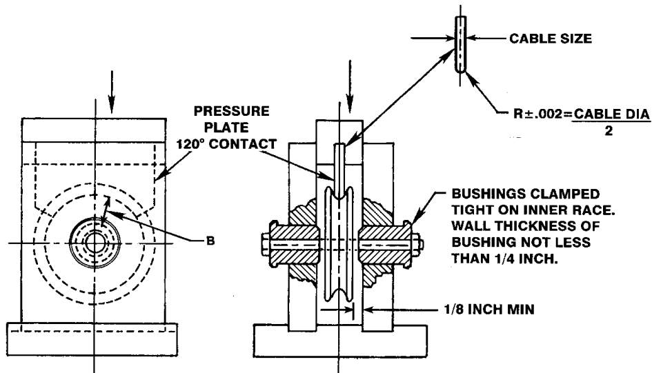
FIGURE 6. Sheave strength test setup.
