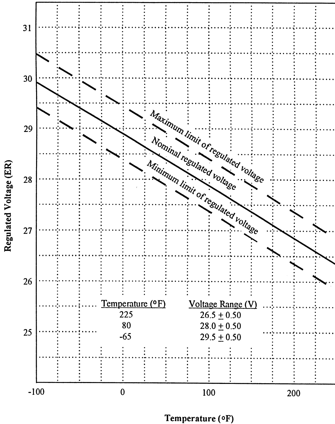
FIGURE 5. Temperature compensation.
