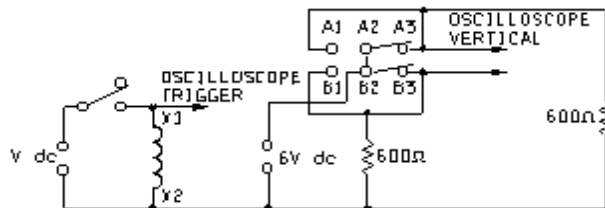
FIGURE 5. Typical break before make test circuits.
