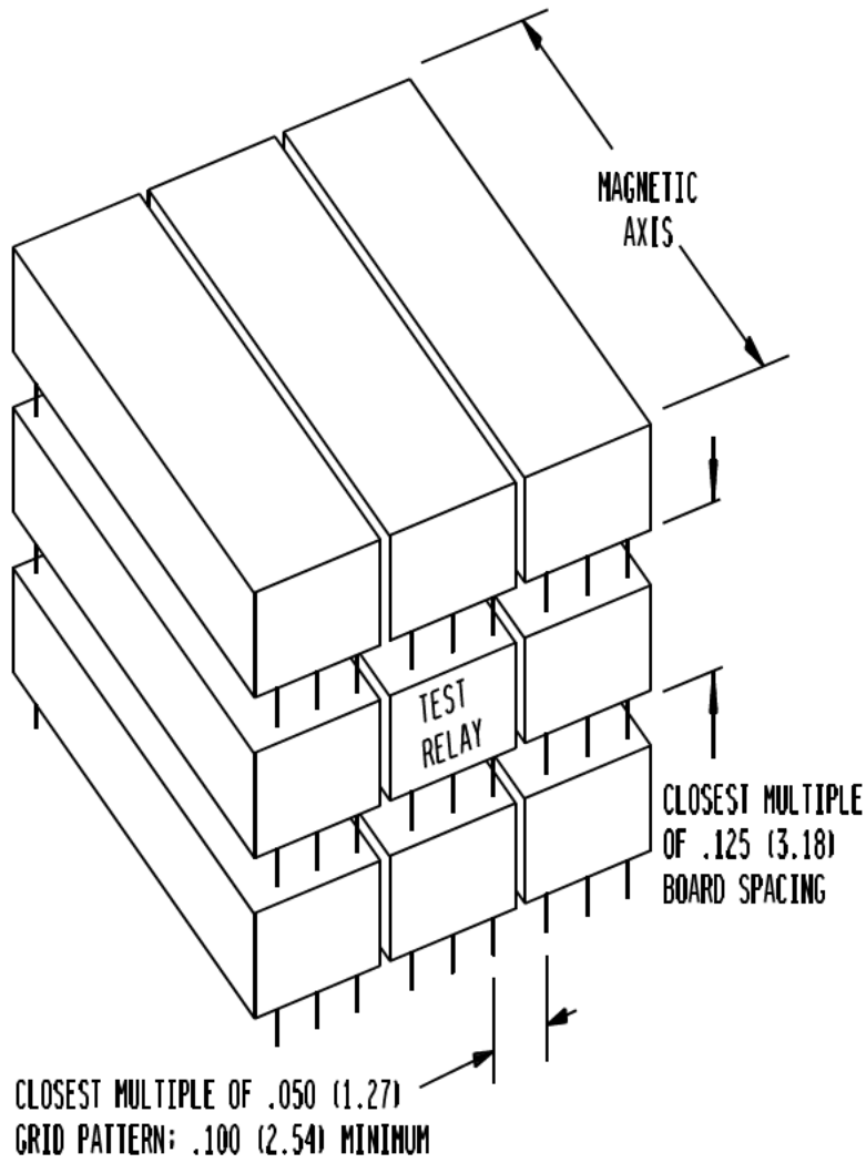
FIGURE 8. Mounting arrays for adjacent similar relays.
