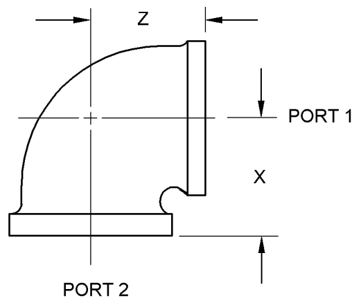
FIGURE 1. 90° reducing elbow.
