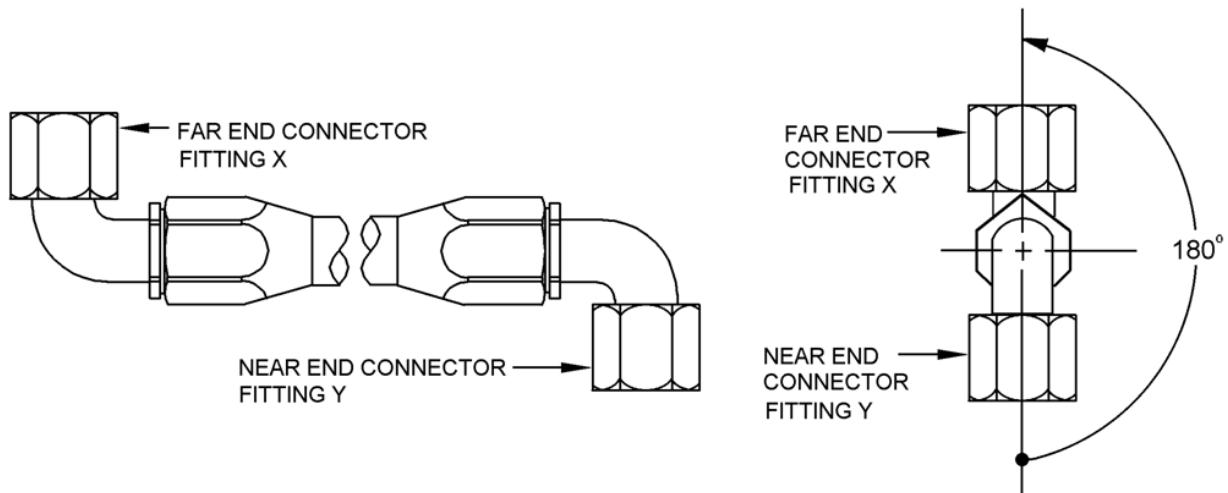
FIGURE 2. Angular displacement .
