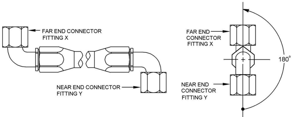
FIGURE 2. Angular displacement .
