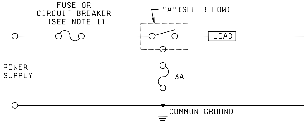
a. Test set-up for single pole switches.
