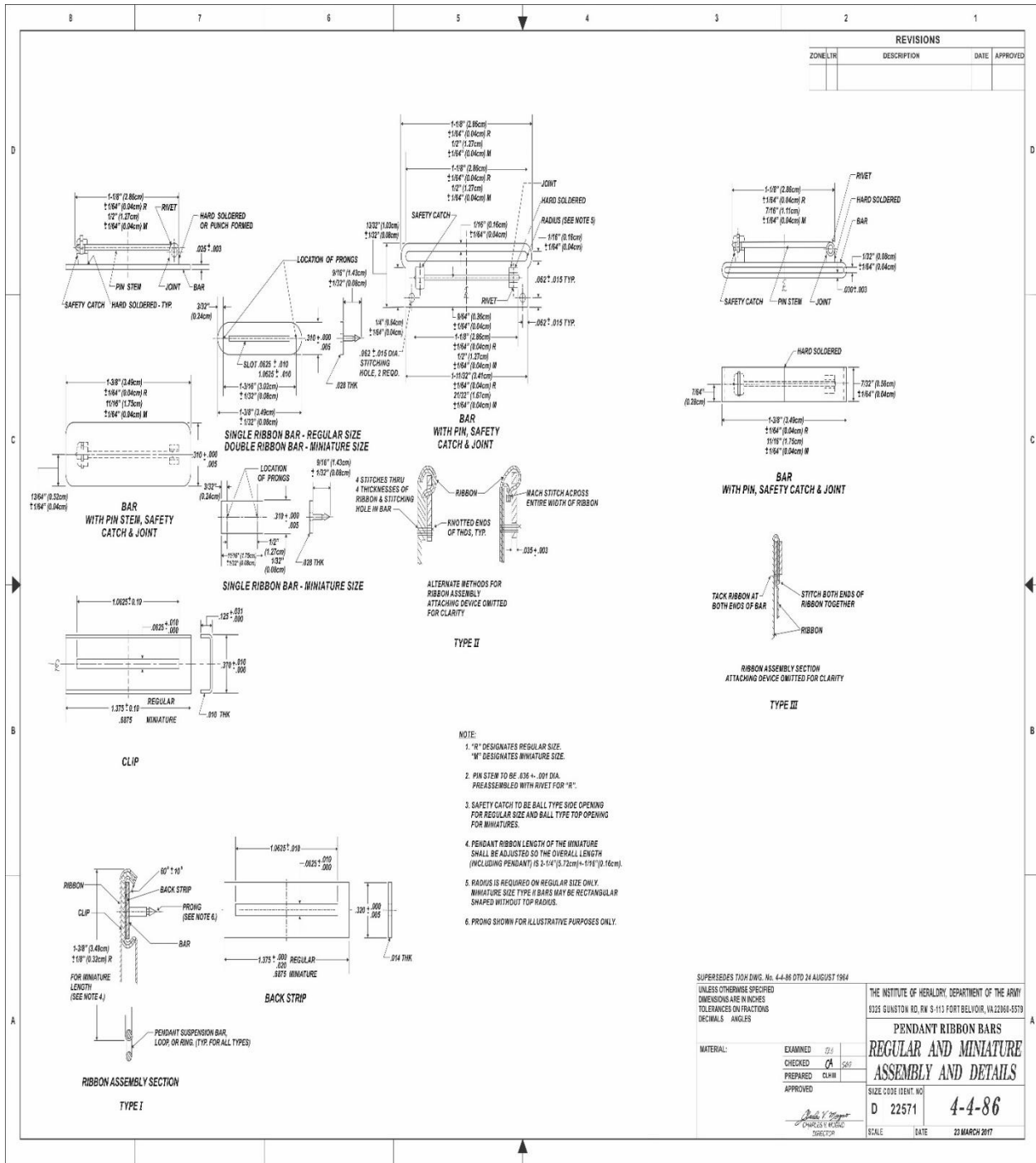
FIGURE 1. Pendant ribbon bars, regular and miniature assembly and details.
