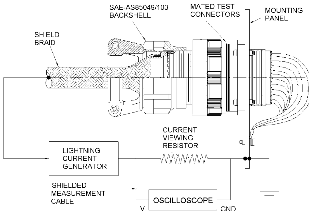
FIGURE 33. Indirect lightning strike test setup.
