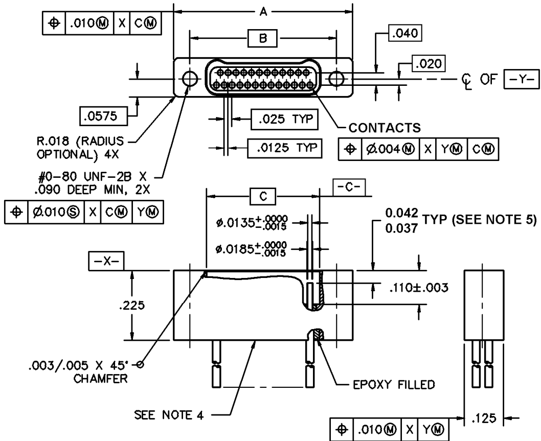
FIGURE 1. Nano connector dimensions and configurations
