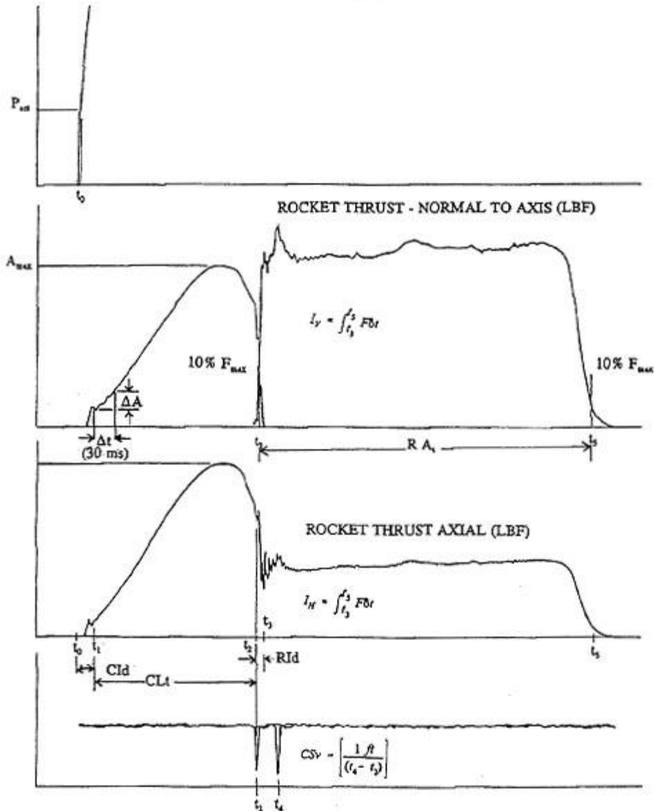
FIGURE 1. Thrust/time Curves
