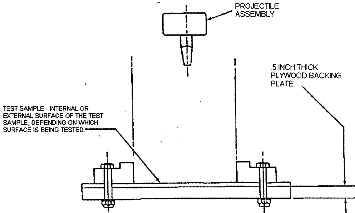
FIGURE 12. Impact chisel.
