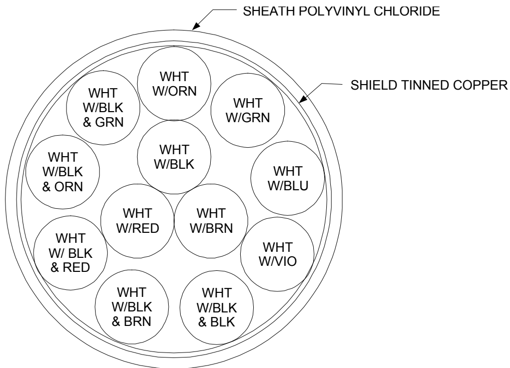
FIGURE 1. Cable configuration.
