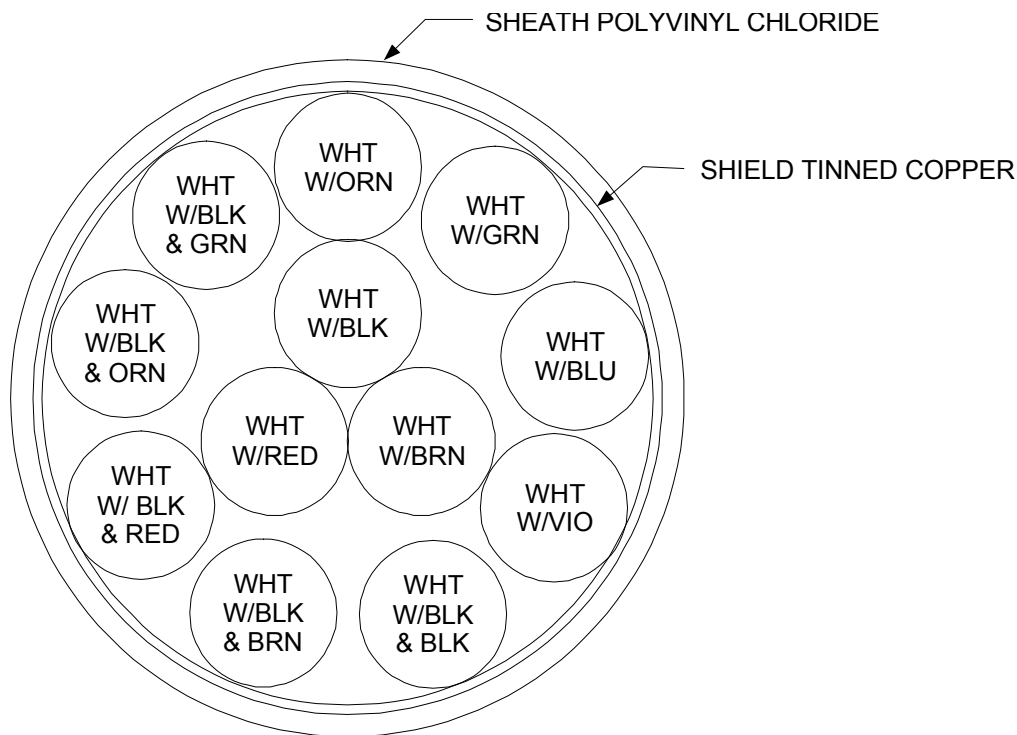
FIGURE 1. Cable configuration.
