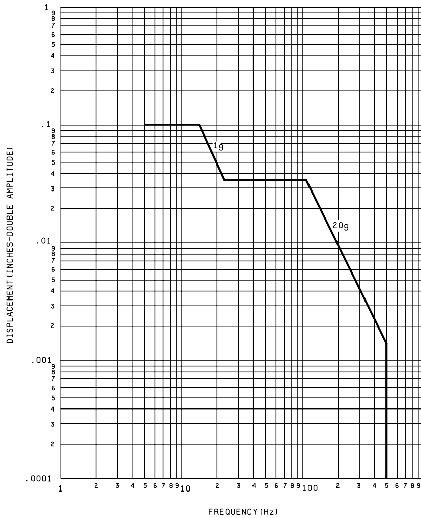
FIGURE 2. Vibration test curve.
