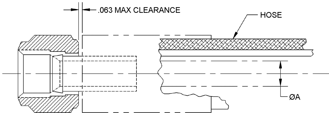
FIGURE 1. Hose assembly.
