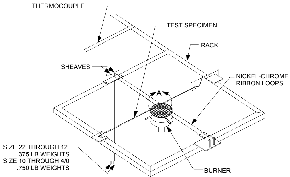
FIGURE 1. Flame test fixture.
