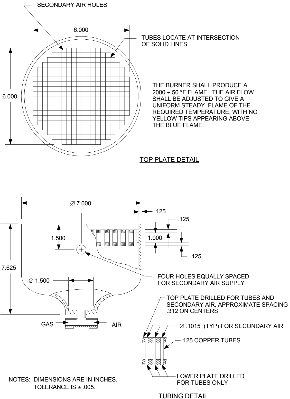
FIGURE 2. Burner details.
