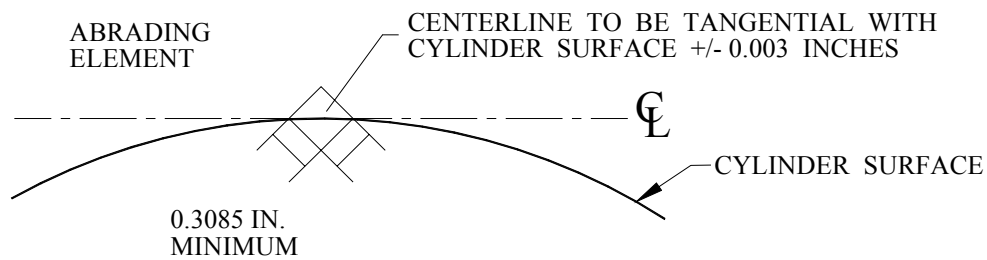
FIGURE 2. Diagram of abrading machine for the abrasion resistance test.
