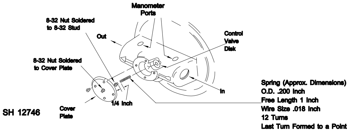
FIGURE 10. Detail drawing of zero pressure governor modification.
