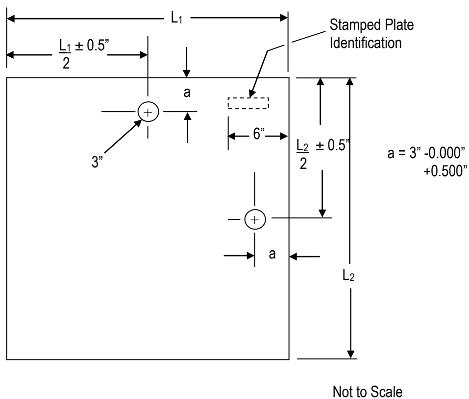
FIGURE A-1. Lifting holes for ballistic acceptance test plates 2.751 through 6.25 inches thick.
