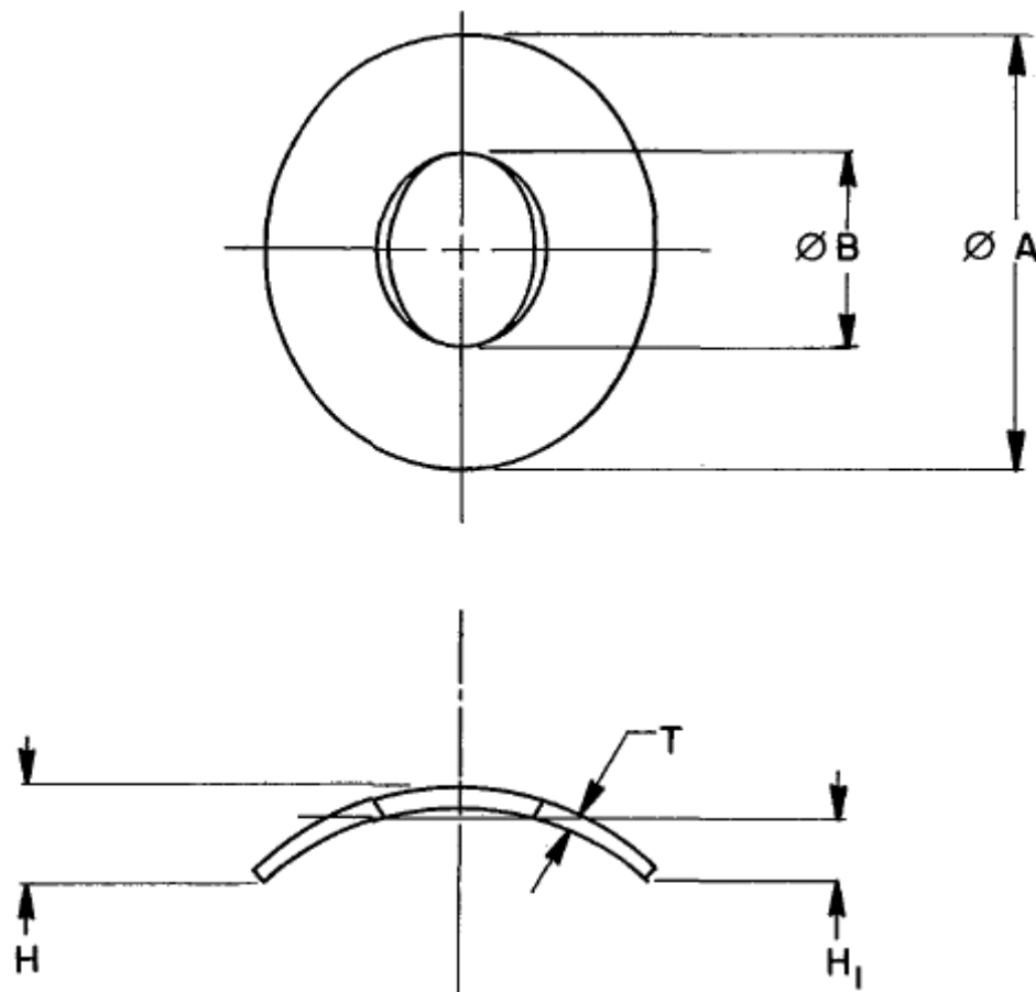
FIGURE 1. WASHER, SPRING TENSION, CURVED, COPPER-BERYLLIUM.
