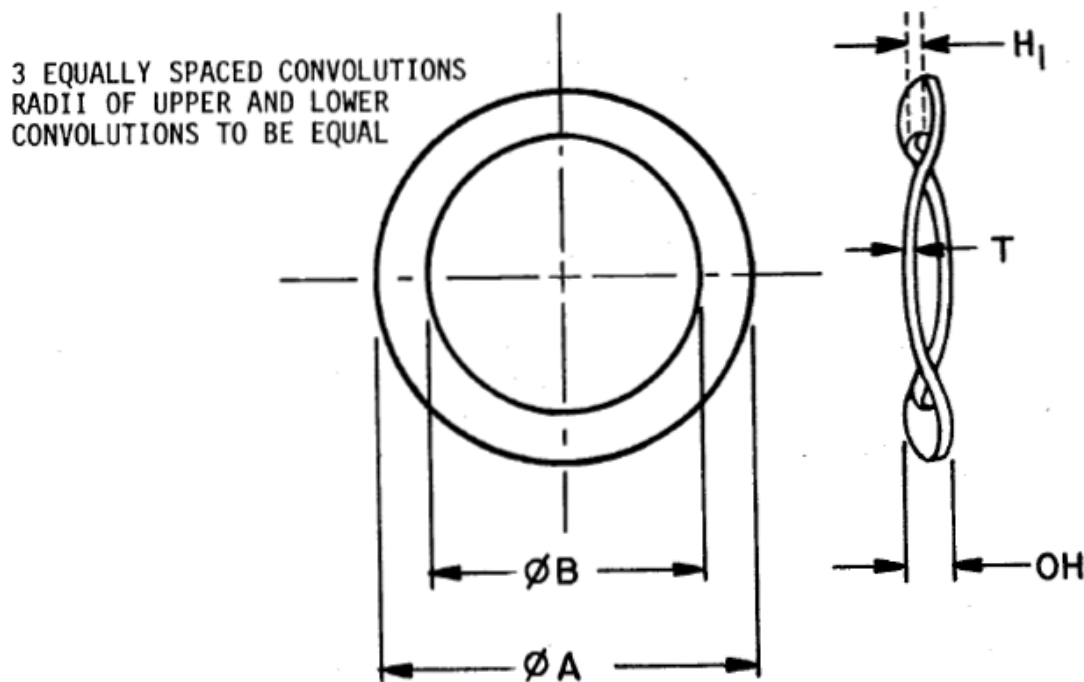
FIGURE 1. WASHER, SPRING TENSION, WAVE, SPRING STEEL.
