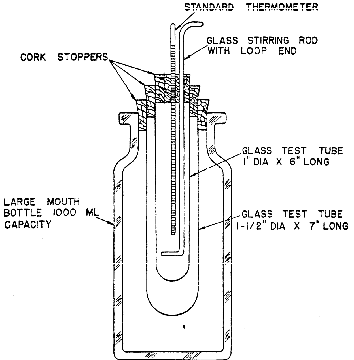
SOLIDIFICATION POINT APPARATUS
