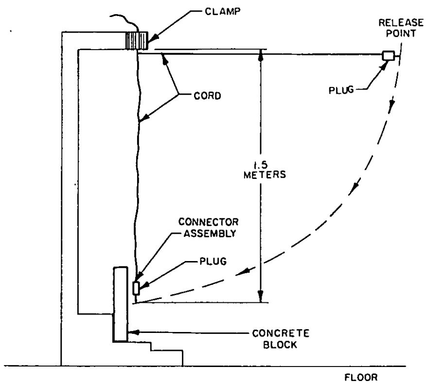
FIGURE 1. Impact test facility.
