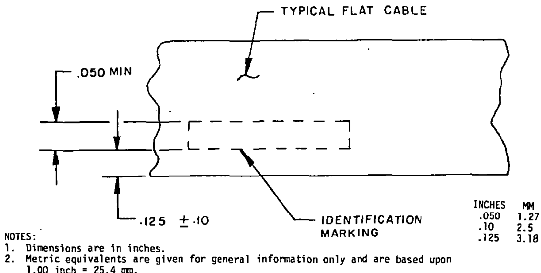
FIGURE 1. Identification marking.
