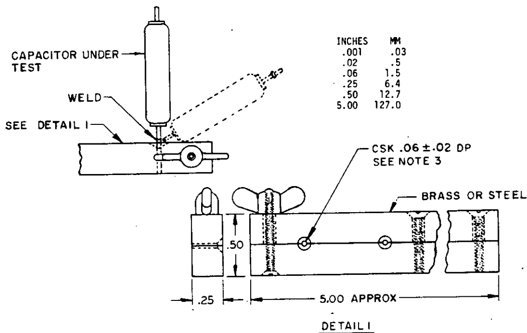
FIGURE 1. Test block fixture for wire-lead bend test.
