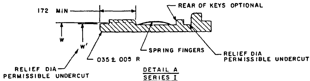
FIGURE 1. Connector intermateability dimensions.
