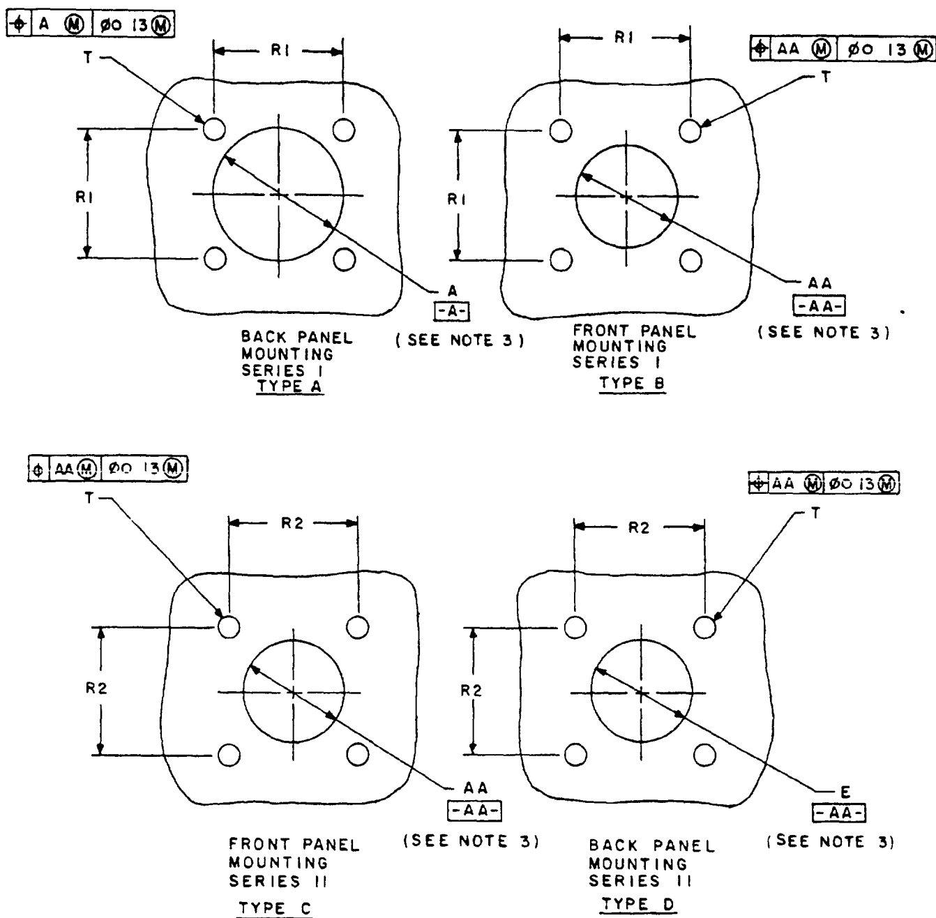
FIGURE 5. Recommended panel dimensions.
