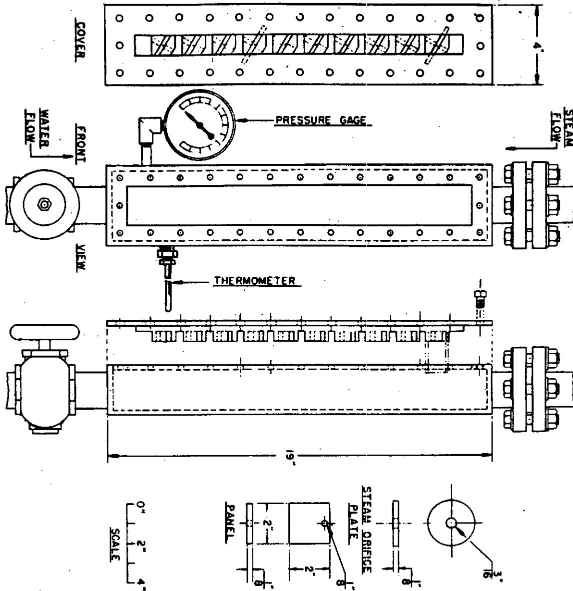
Figure 8 - Hot water - low pressure steam removability apparatus.
