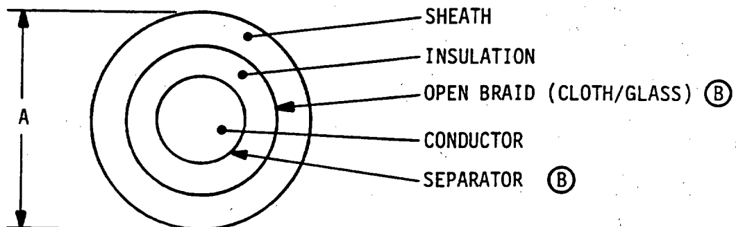
FIGURE 1. Configuration.
