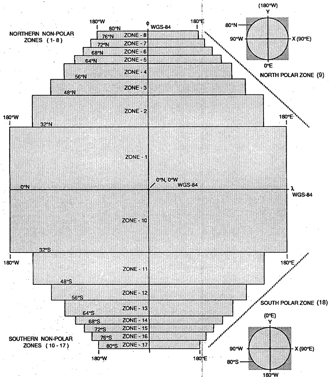
FIGURE 22. ARC system zone layout.
