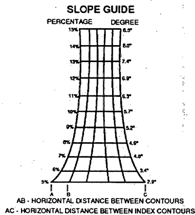
FIGURE 8. Slope diagram.
