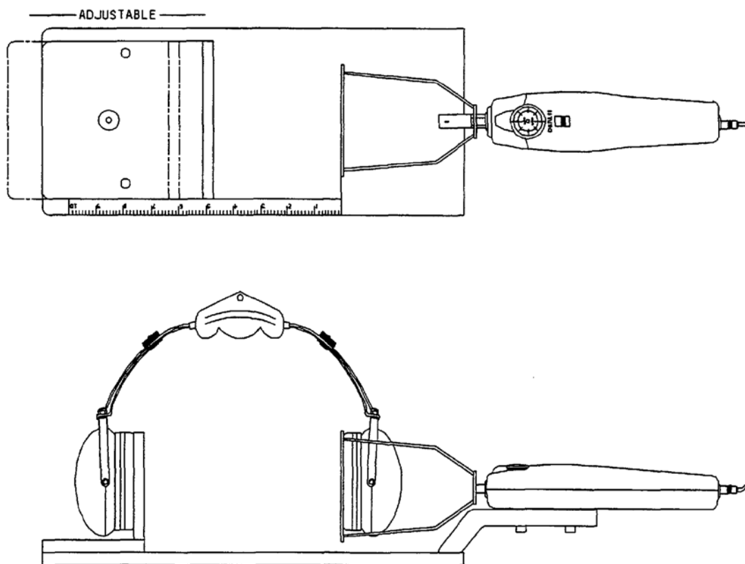
FIGURE 4. Example of headband pressure device.
