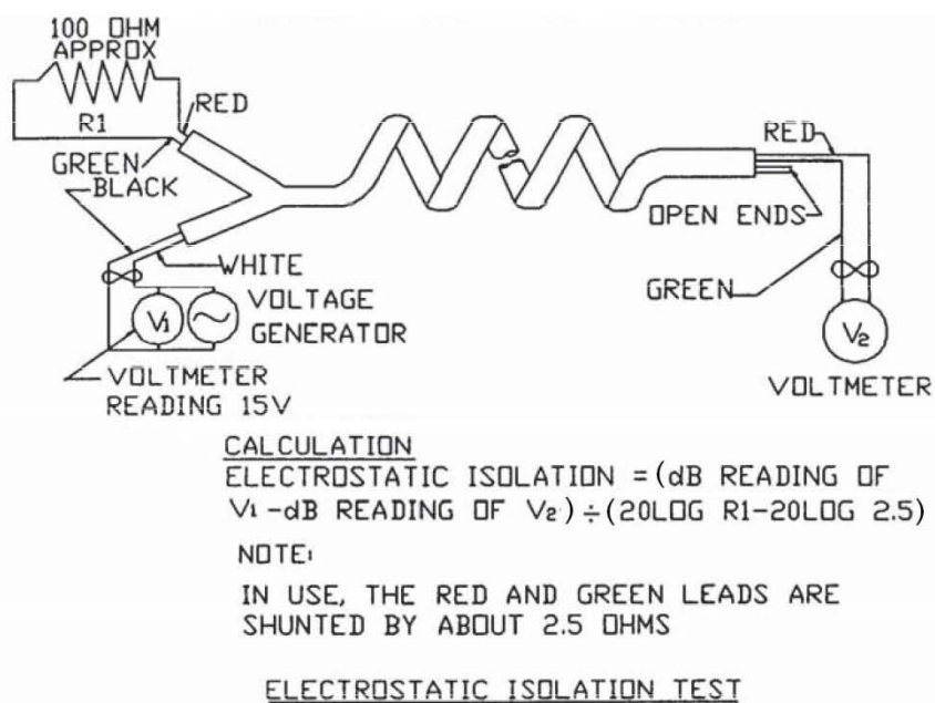
FIGURE 6. Isolation test setup.
