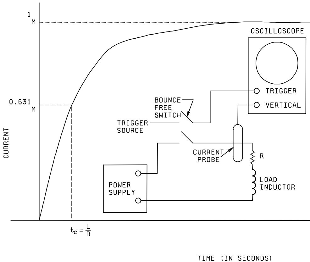
Figure 3. DC inductive load (inductive current rise time curve).
