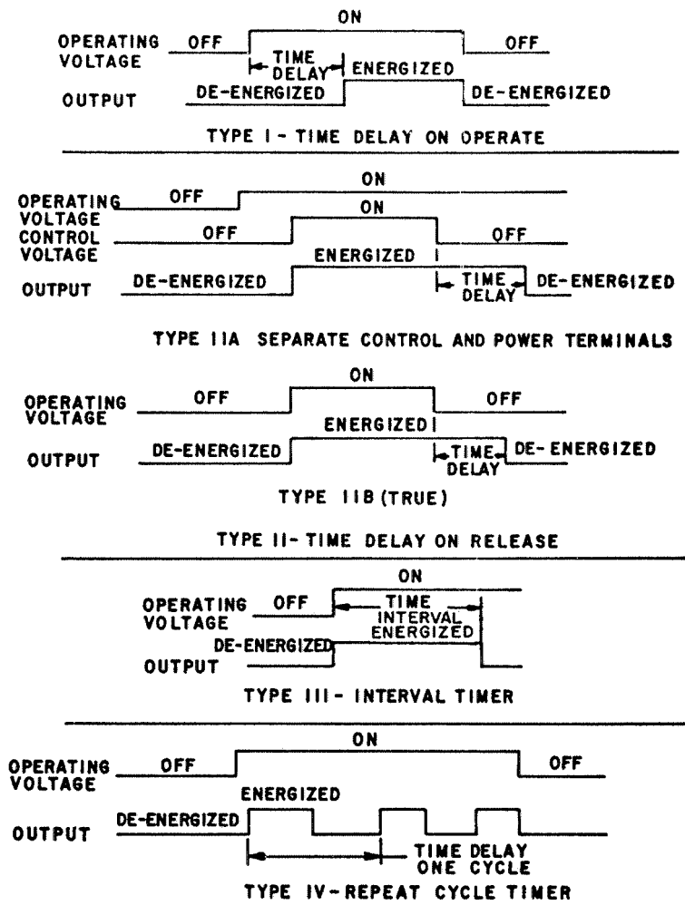
FIGURE 4. Relay timing diagrams.
